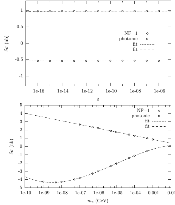
Fig. 1. Differences between the \sigma_{\text{SV}}^{\alpha^2} of BabaYaga@NLO and the \mathcal{O}(\alpha^2) calculations of Ref. [16] (photonic) and of Ref. [17] ( N_F = 1 ), as a function of the infrared regulator (top) and of a fictitious electron mass (bottom).
