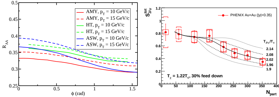
Fig. 3. Left: R_{AA} as a function of azimuthal angle at p_T = 10 GeV/c (solid line) and p_T = 15 GeV/c (dashed line) for all three approaches in the 20–30% centrality bin (figure taken from [43]). Right: J/\psi survival probability as function of N_{\text{part}} for different J/\psi dissociation temperatures (figure taken from [49]).
