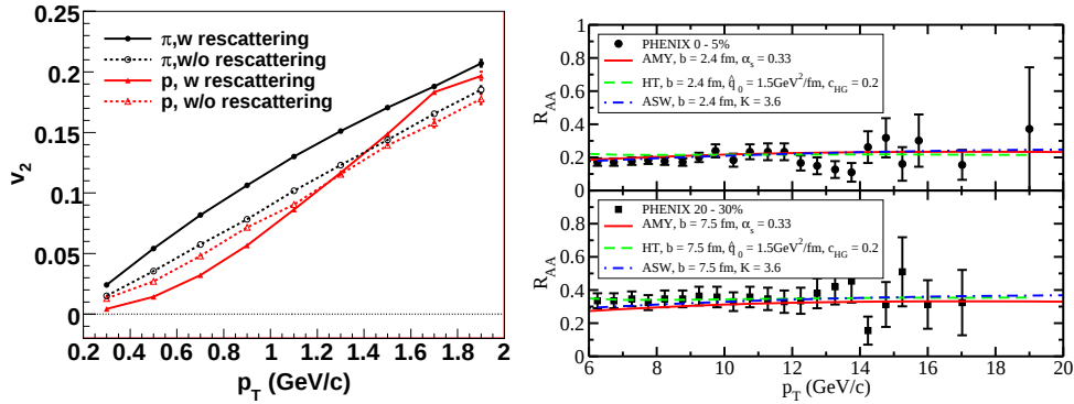
Fig. 2. Left: transverse momentum dependence of v_2 for protons and pions in the hydro+cascade model (figure taken from [19]). The hadronic phase is responsible for the mass-splitting between protons and pions. Right: Nuclear modification factor R_{AA} in Au–Au collisions at 0–5% (top) and 20–30% (bottom) centrality calculated in the ASW, HT and AMY approaches compared to data from PHENIX [44] (figure taken from [43]).
