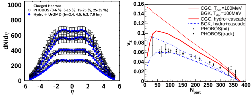
Fig. 1. Left: Centrality-dependence of charged particle pseudo-rapidity distributions in the Hydro+UrQMD approach (figure taken from [16]). Right: Centrality dependence of the elliptic flow coefficient v_2 for different initial conditions and treatment of the hadronic phase (figure taken from [15]).
