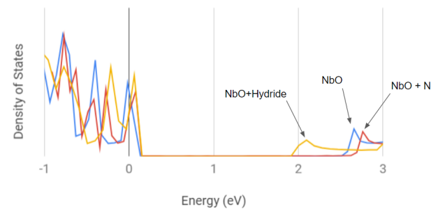
Figure 6: Example density of states calculations for the same monolayer oxide surface with different sub-surface impurities.
