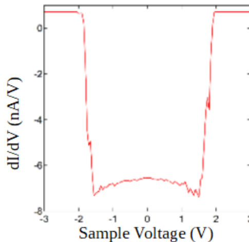
Figure 5: Example dI/dV measurement by the Sibener group.
