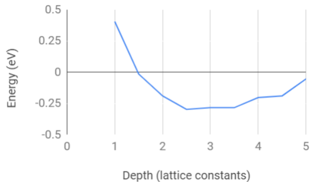
Figure 8: Calculated energy for nitrogen interstitials as a function of depth in lattice constants beneath the surface.
