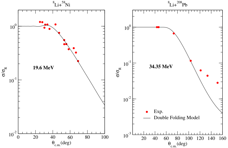
Fig. 3. Elastic scattering angular distributions for {}^8\text{Li}+{}^{58}\text{Ni} , and {}^8\text{Li}+{}^{208}\text{Pb} . The solid lines show the double folding model results, while the circles show the experimental data, which have been taken from [11, 13].
