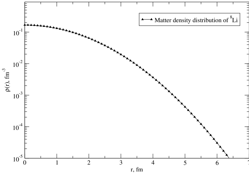
Fig. 1. The matter density distribution of ^8\text{Li} nucleus within the GG density distribution.
