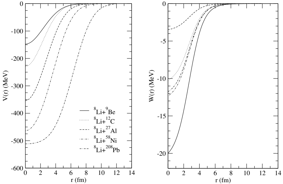
Fig. 4. The shapes of the real and the imaginary potentials of the nuclear potential of ^8\text{Li} which interacts with different target nuclei.
