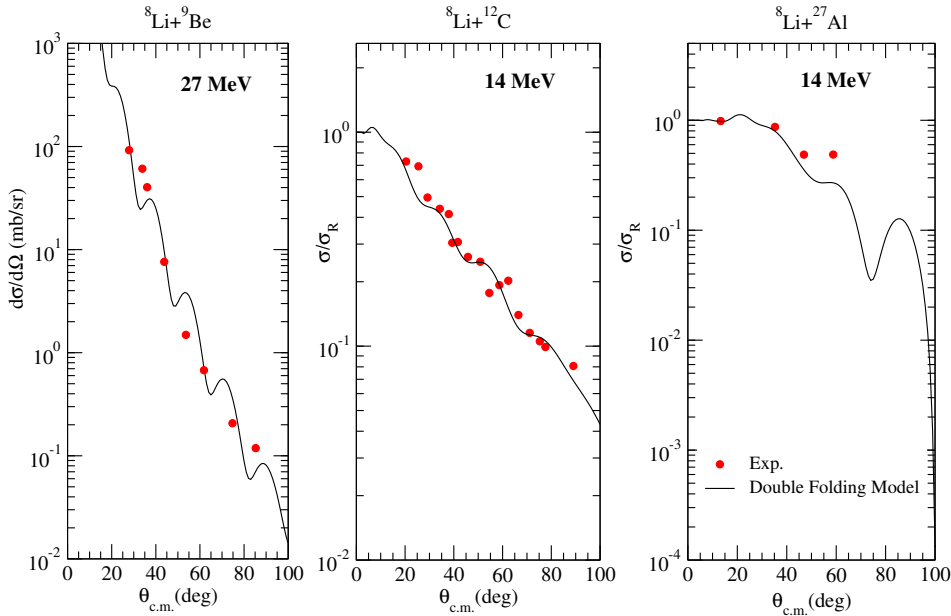
Fig. 2. Elastic scattering angular distributions for ^8\text{Li}+^9\text{Be} , ^{12}\text{C} , and ^{27}\text{Al} . The solid lines show the double folding model results, while the circles show the experimental data, which have been taken from [11, 12].
