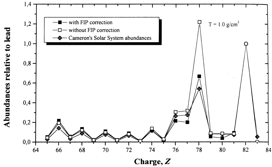
Fig. 1. Abundances relative to lead of UH cosmic ray ions in the Earth's neighbourhood obtained by propagating Solar System type source abundances (Cameron, 1982), also shown in the figure, with and without the FIP correction.
