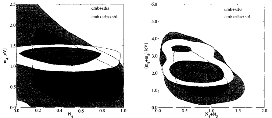
Figure 2: Left: (3 + 1) analysis – Two dimensional marginalized 68% and 95% confidence level regions in the plane N_4 vs. m_4 for the different combinations of datasets. Right: Reduced (3 + 2) analysis – Two dimensional marginalized 68% and 95% confidence level regions in the plane (N_4 + N_5) vs. (m_4 + m_5) for the different combinations of datasets. Plots taken from Achidiacono et al. (2013).
