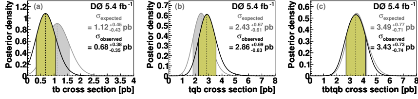
Figure 1.: The expected (grey) and observed (yellow) posterior probability densities for (a) tb , (b) tqb and (c) tbtqb production. The shaded bands indicate ranges for 68% C.L. for the peak values.
