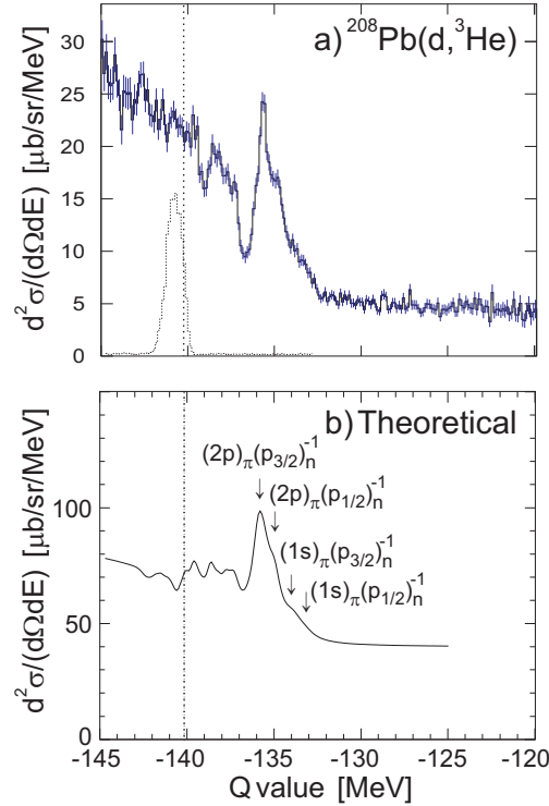
Fig. 1. The experimental Q value spectrum obtained in the ^{208}\text{Pb}(d, {}^3\text{He}) reaction at the present stage of analysis (a) in comparison to the theoretical prediction by Hirenzaki et al. [3]. The dotted line at Q = -140.15 MeV indicates the \pi^- binding threshold. The p(d, {}^3\text{He})\pi^0 peak used for the Q value calibration is also shown.
