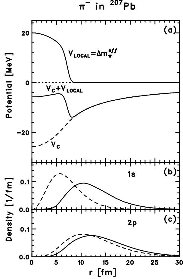
Fig. 4. The \pi^- mass shift and local potential (top) and the \pi^- densities in the 1s and 2p state (bottom) as a function of the radius. The dashed curves are obtained for a pure Coulomb potential.
