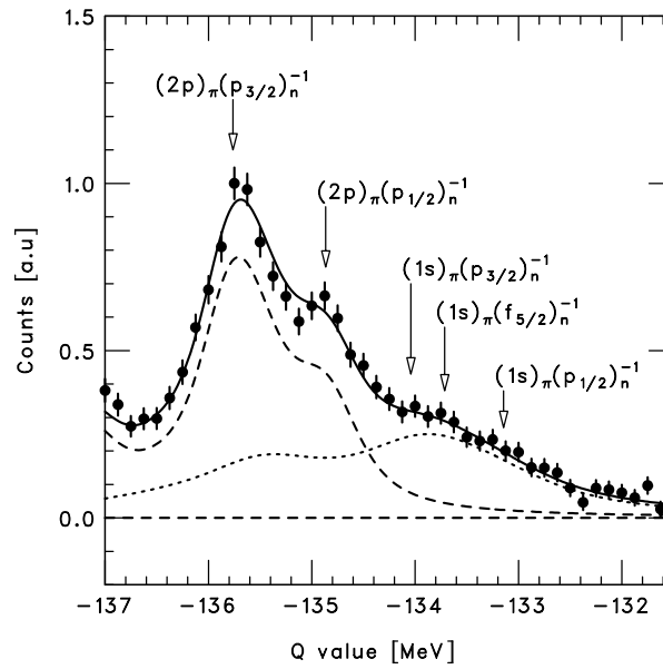
Fig. 2. Decomposition of the peak region of the experimental Q value spectrum of the ^{208}\text{Pb}(d,^3\text{He}) reaction into the 2p component (dashed curve) and the 1s component (dotted curve), using the shape of the theoretical calculation [3]. The best fit is obtained if the 1s/2p intensity ratio is 2.5 times the theoretical ratio.
