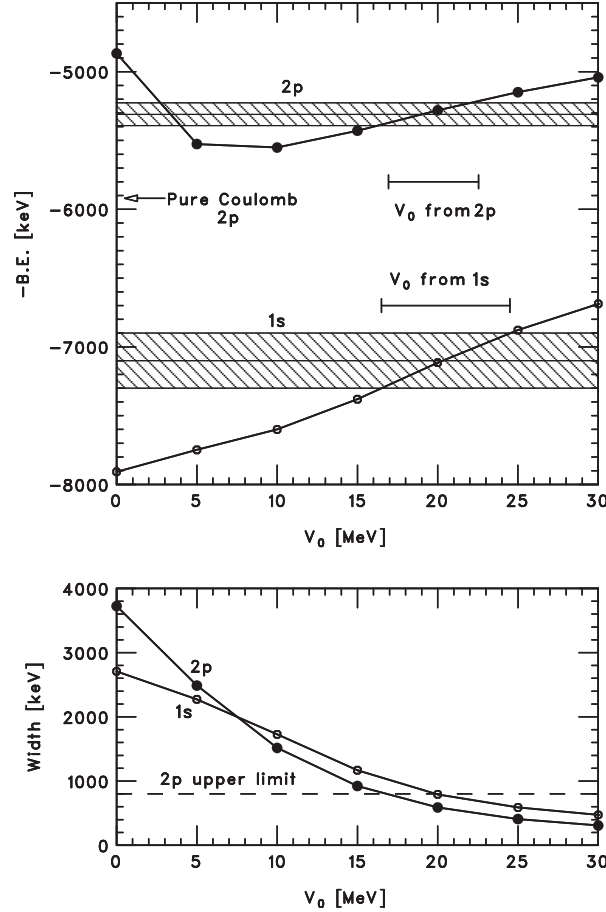
Fig. 3. Relation of the local potential V_0 and the binding energies of the pionic 2p and 1s states (upper part) and of the width of both states (lower part).
