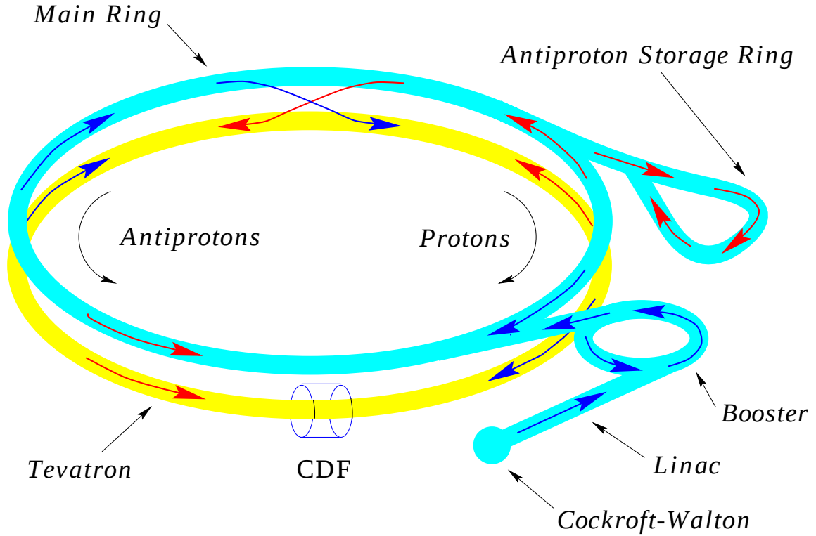
FIG. 9. The Fermilab Accelerator showing the stages of acceleration.
