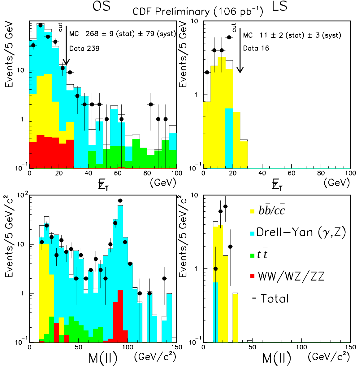
FIG. 41. The E_T and M(\ell, \ell) distributions displaying data and the expected Standard Model background using ISAJET 7.16 [61] with MRSD0' as the parton density function at Stage-6. The arrow displays where the E_T cut is made. One can see that there are no like-sign dilepton events after E_T \geq 25 GeV.
