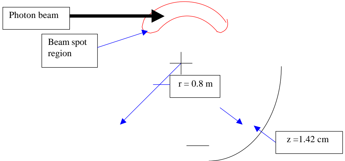
Figure 1. Target wheel schematic
