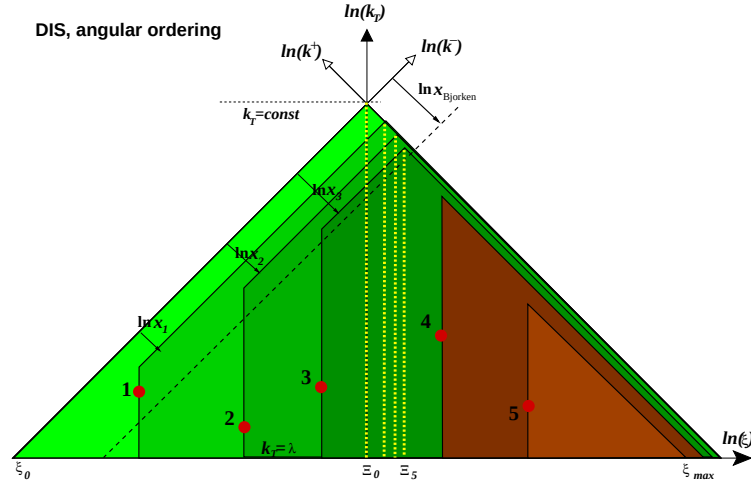
Fig. 6. The phase space of MMC/CMC with the angular ordering parton shower based on CCFM-like evolution. The entire triangle represents the so-called “current region”. The proton fragmentation region is to the left of the triangle. The right-hand side part of the triangle is populated by the final state gluonstrahlung.
