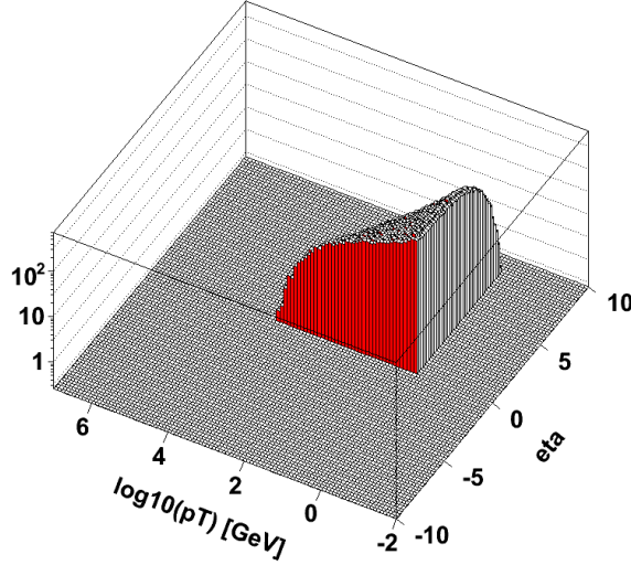
Fig. 3. The distribution of all gluons emitted from a single proton from CMC. The sharp boundaries of rapidity and minimum k^T are clearly visible.
