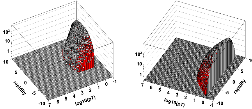
Fig. 4. The CMC results for the distribution of all gluons emitted from two proton beams. In the left-hand side plot rapidity of the W boson is fixed to -3 while in the right-hand side plot it is unrestricted.
