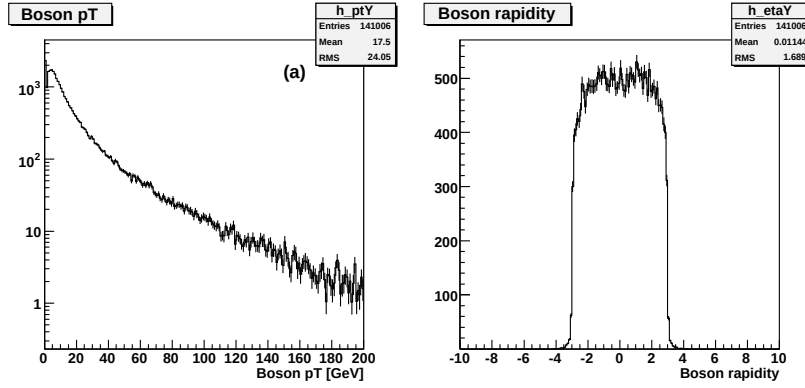
Fig. 5. The transverse momentum and rapidity distribution of the electroweak boson from the double CMC prototype program.
