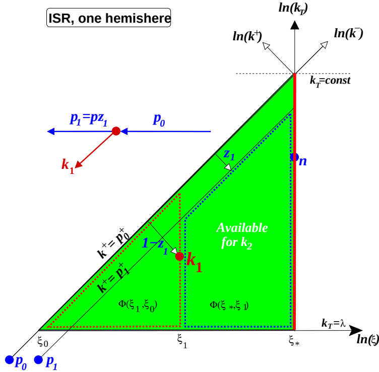
Fig. 2. The phase space of the single gluon emission.
