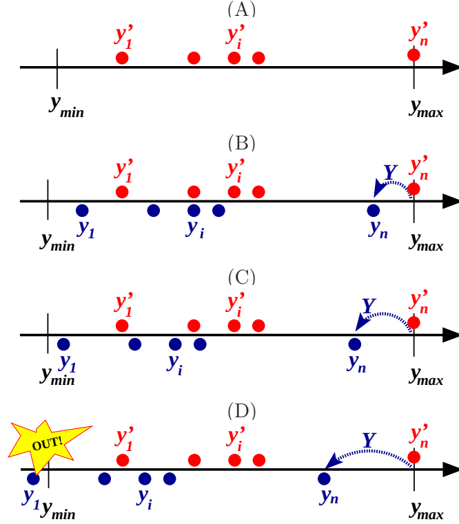
Fig. 1. The linear shift y'_i \rightarrow y_i = y'_i - Y(y'_1, y'_2, \dots, y'_n) in the CMC algorithm illustrated in four steps: (A) begin with y'_i such that one of them y'_n \equiv y_{\max} , (B), (C) shift y'_i \rightarrow y_i by Y , where Y solves the constraint condition x = \sum u_i(y_i) ; Y is therefore a complicated function of all y'_i . (D) Sometimes the smallest y'_i is shifted out of the phase space, below the IR limit y_{\min} . Such an event gets zero MC weight.
