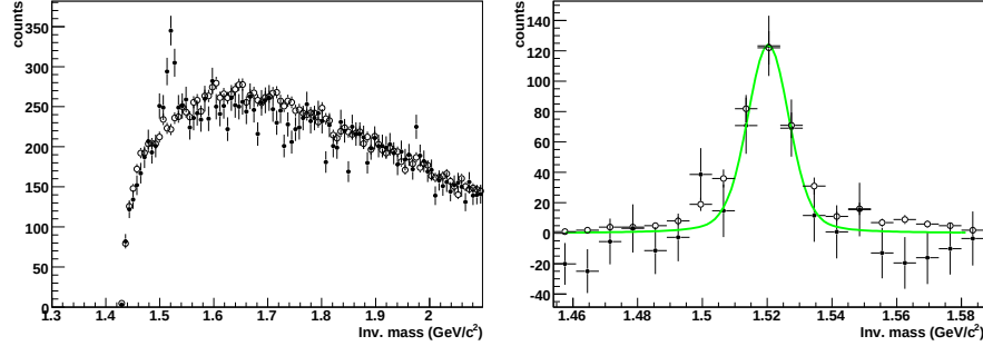
Fig. 2. Left: Invariant mass distribution of all charged pK pairs (black points) in the case of a perfect particle identification, for 6 \times 10^4 PYTHIA pp collisions, and combinatorial background estimated by the event mixing technique (open points). Right: Invariant mass distribution of \Lambda(1520) obtained after the background subtraction (black points). The open points represent the invariant mass distribution of the true pairs originating from the \Lambda(1520) decay.
