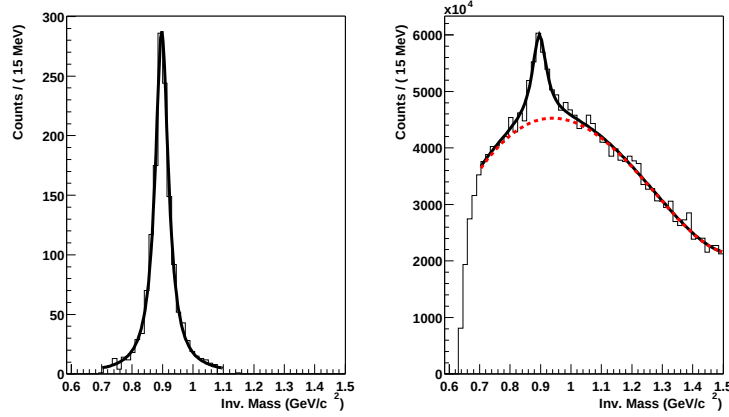
Fig. 1. Invariant mass distribution of the true pairs originating from the K^*(892)^0 and its antiparticle decay (left panel) and from all unlike-sign K\pi pairs (right panel) in case of a perfect particle identification, for 2 \times 10^5 PYTHIA pp collisions. The solid curves are the fit results. The dashed curve in the right part is the polynomial function representing the background.
