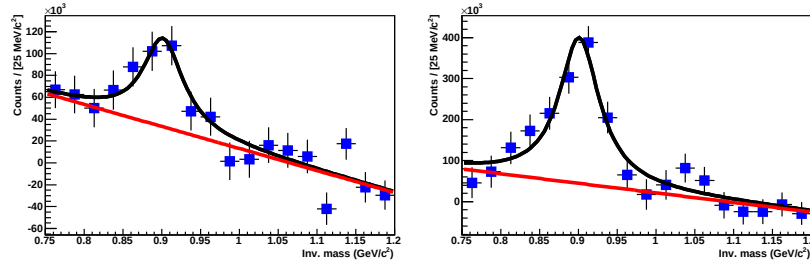
Fig. 4. K^*(892)^0 resonance peak obtained after subtraction of like-sign background, with a perfect PID (left, 3840 HIJING events) and realistic ID (right, 15000 HIJING events). The curves represent a fit by a Breit–Wigner plus a linear background.
