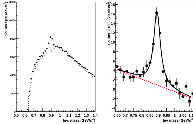
Fig. 3. Left: invariant mass distribution of the K^+\pi^- and K^-\pi^+ pairs in the case of a realistic PID; the dashed line represents the combinatorial background obtained from the event-mixing technique. Right: signal spectrum obtained after the background subtraction. The solid curve is a Breit–Wigner fit to the spectrum whereas the dashed curve is the linear function representing the residual background.
