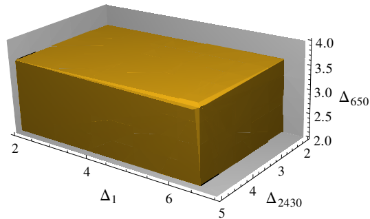
Figure 4.18: Three-dimensional exclusion plot in the octant spanned by the scaling dimensions of the first unprotected scalar in the \mathfrak{R} = \mathbf{1}, \mathbf{650}, \mathbf{2430} representations of \mathfrak{e}_6 with k = 6 and c = \frac{13}{6} . The cutoff used while generating these bounds was \Lambda = 12 .
