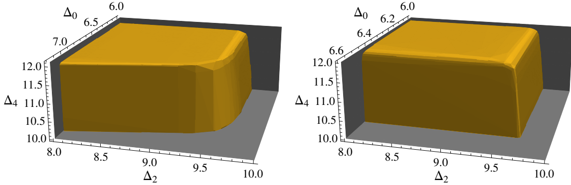
Figure 5.10: Simultaneous bounds on the spin 0, 2, 4 superconformal primary dimensions for a cutoff of \Lambda = 22 . These bounds are for the central charge corresponding to the A_1 theory ( c = 25 ), and are obtained with (left) and without (right) the addition of the short multiplet \mathcal{D}[0, 4] . The allowed region is inside of the region delimited by the yellow surface.
