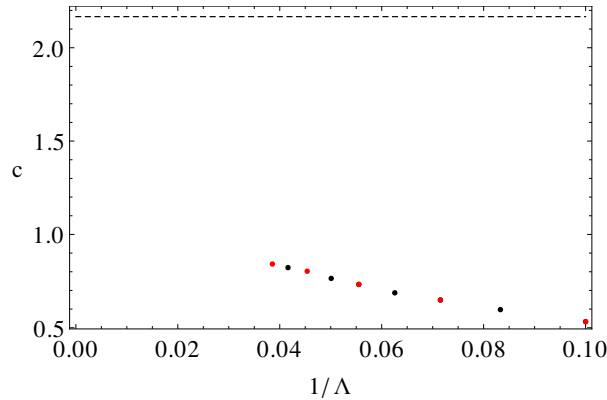
Figure 4.13: Lower bounds on c for a theory with \mathfrak{e}_6 flavor symmetry and k = 6 as a function the inverse cutoff \Lambda . The red dots correspond to derivatives 10, 14, \dots , 26, while the black dots show the remaining even values of \Lambda ranging from 10 to 24. The dashed line at c = \frac{13}{6} marks the central charge of the rank one \mathfrak{e}_6 theory.
