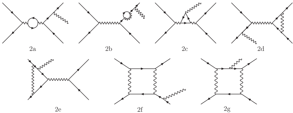
Fig. 1. Representative one-loop diagrams for e^-e^+ \rightarrow e^-e^+\gamma .
