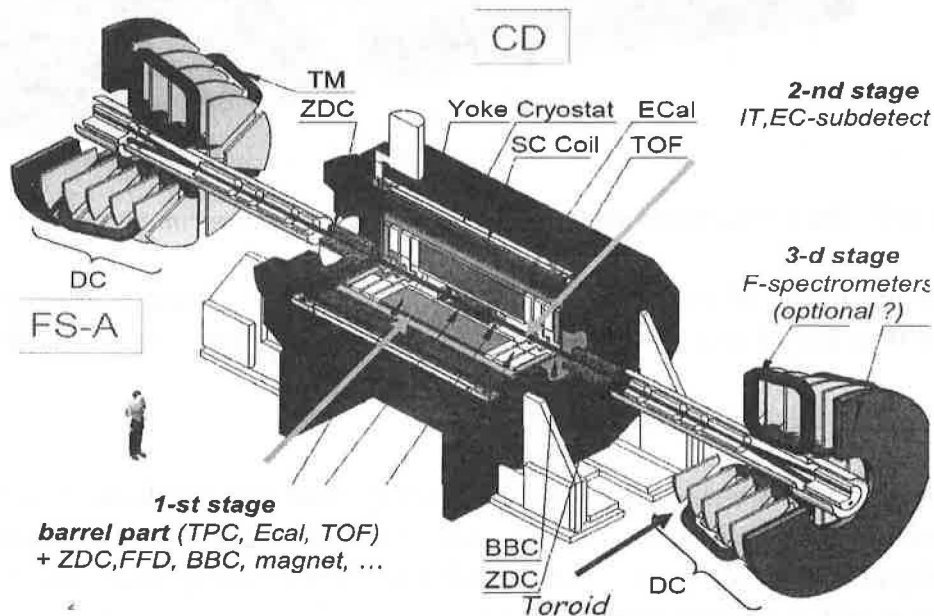
Figure 4. General view of the MPD, and sets of sub-detectors to be put in operation at different stages.
