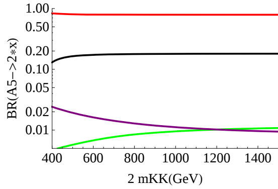
Figure 4.9: Branching ratios of the heavy A_\mu^{2,0} as a function of 2 m_{KK} in GeV: SM jet , SM tops, l \bar{l} , \nu \bar{\nu} . The contributions of Z_L h and W_L^+ W_L^- channels are smaller than 0.01%.
