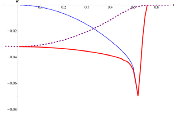
Figure 5.2: Contribution to \kappa from a bulk fermion in GHU as a function of the bulk mass c , 1/R = 1 TeV, and m_H = 130 GeV. The dotted blue line represents the contribution of the light mode (deviation from the SM one), the dashed purple line is for the KK tower and the thick red line corresponds to the sum of both.
