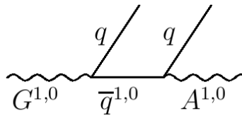
Figure 4.1: Decay chain of the heavy gluon G^{(1,0)} .
