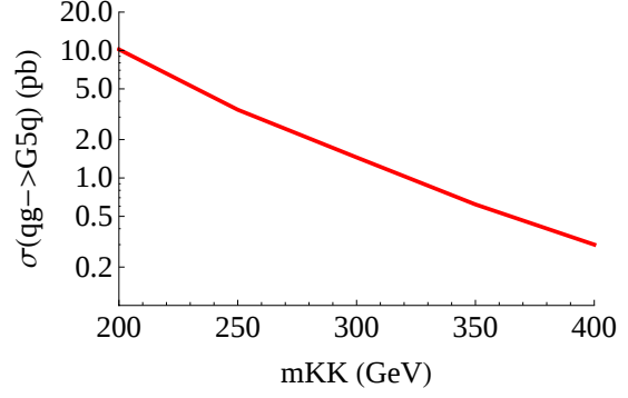
Figure 4.21: G_{\mu}^{2,0} single production through q g \rightarrow G_{\mu}^{2,0} q : 7 TeV cross-section.
