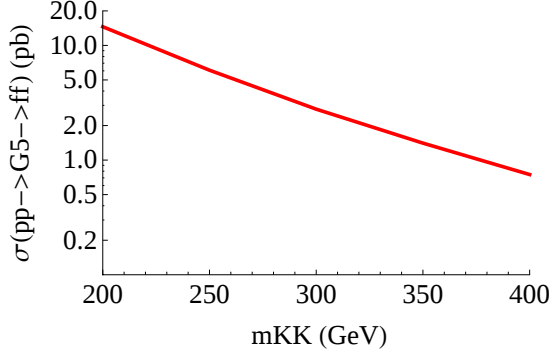
Figure 4.20: G_{\mu}^{2,0} single production through q \bar{q} \rightarrow G_{\mu}^{2,0} \rightarrow f \bar{f} : 7 TeV cross-section.
