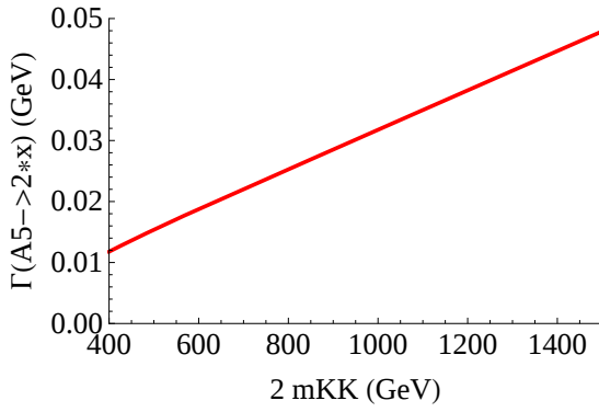
Figure 4.8: Inclusive decay width of the heavy A_\mu^{2,0} as a function of 2 m_{KK} in GeV.
