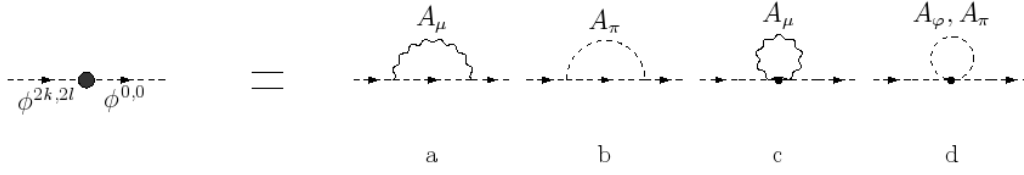
Figure 3.5: Scalar mixings generated by gauge loops.
