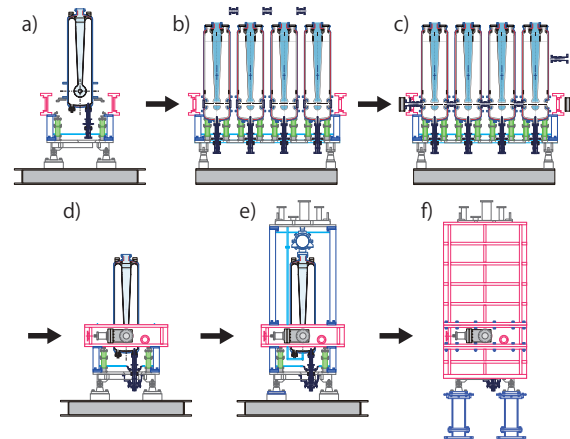
Figure 6: Assembly procedure of SRILAC cryomodules.
