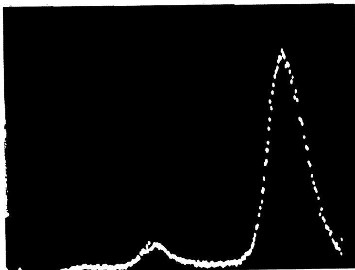
OBSERVED PULSE HT DISTRIBUTION USING F_{e55} SOURCE
