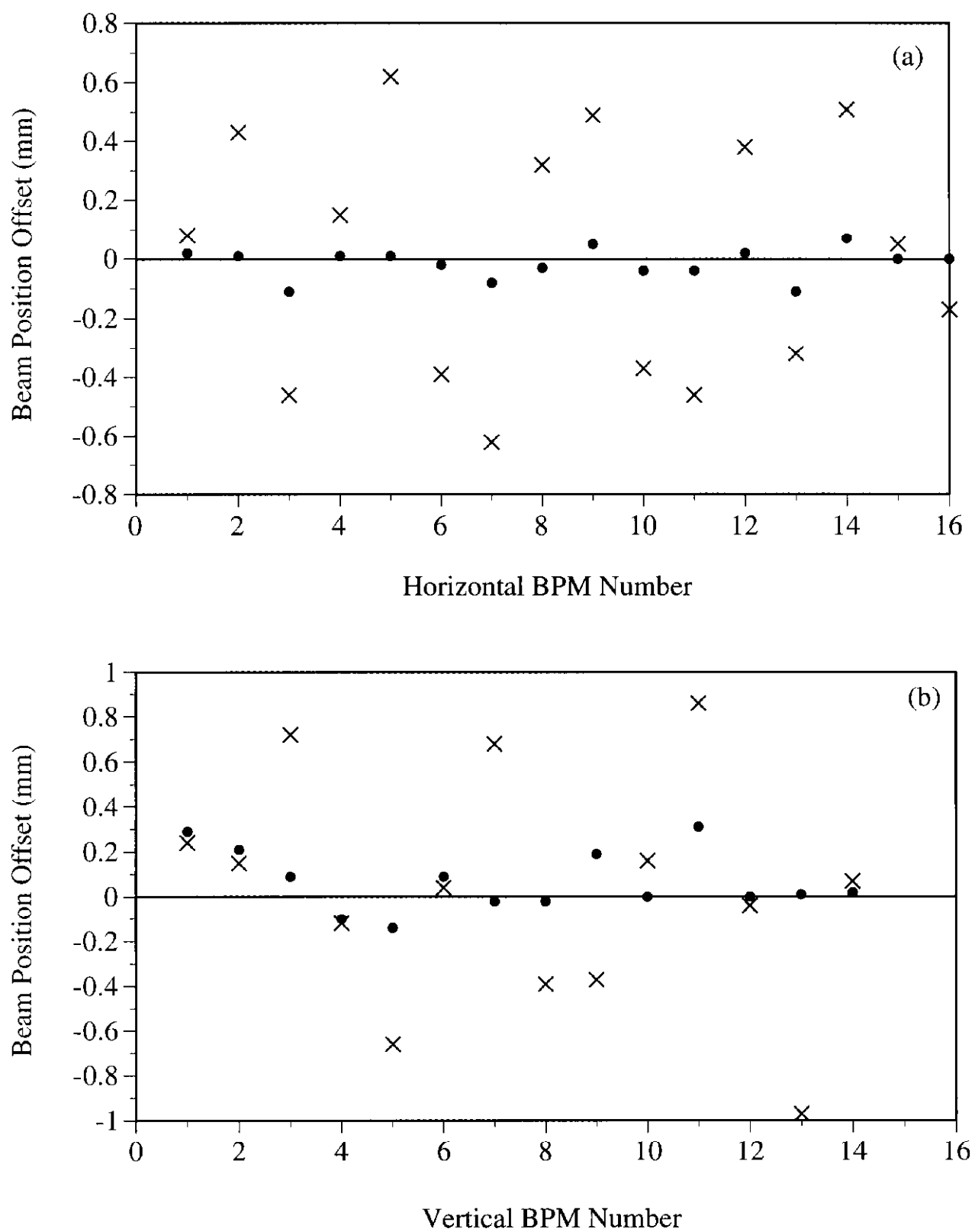
Fig. 1. Initial (X) and Final (•) beam position offsets for (a) the horizontal plane, and (b) the vertical plane.
