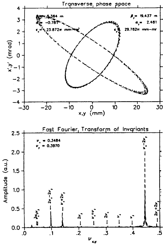
Figure 2. Transverse Phase Space and Resonance Spectrum of the "ideal" LEB lattice
