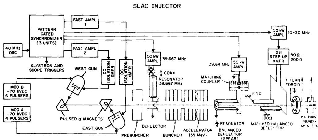
Fig. 1. Injector system block diagram.
