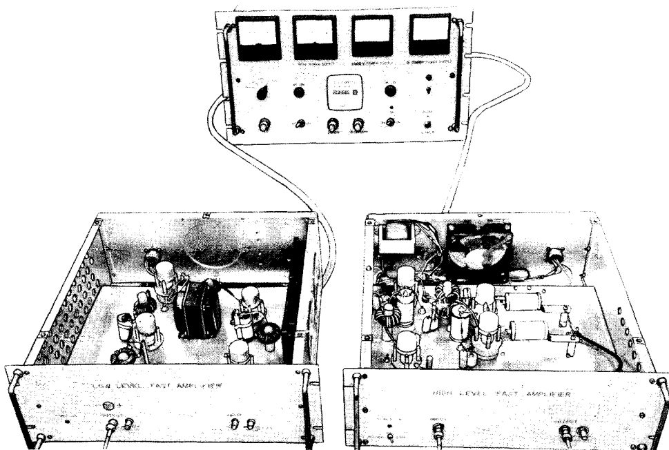
Fig. 3. Fast pulse amplifier system.
