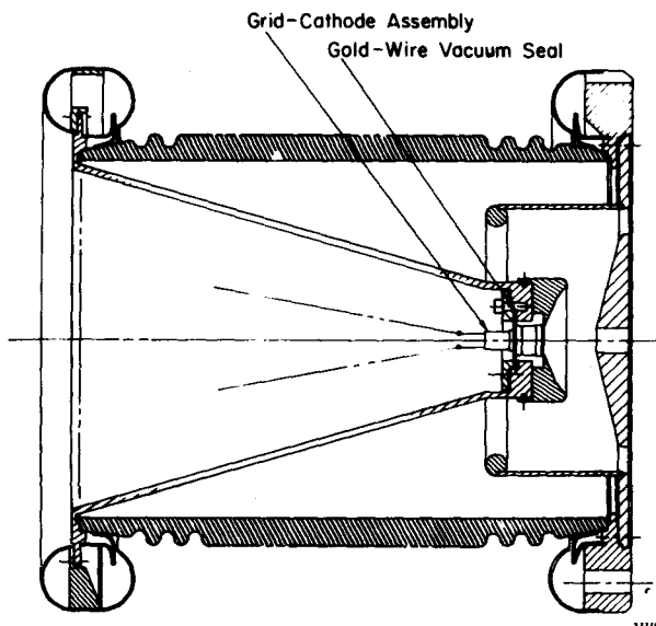
Fig. 2. High current, fast pulse gun.
