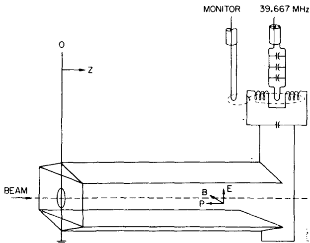
Fig. 4. Downstream deflector schematic.
