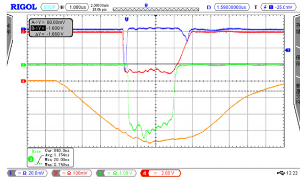
Figure 6: Incident wave (pink), reflected wave (blue), target current (green) and the voltage of electron gun(orange).
