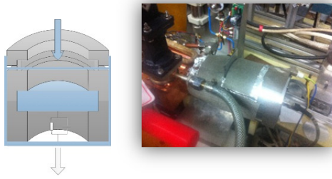
Figure 7: The design of the Faraday cup and its measurement position.
