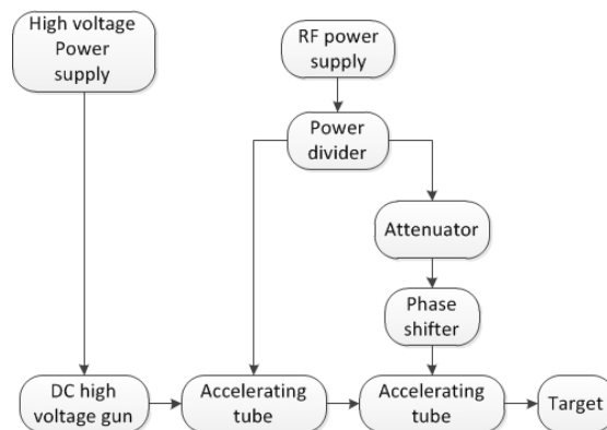
Figure 1: Schematic diagram of the linac system.
