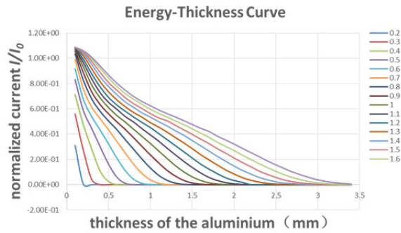
Figure 2: simulation data of the current ratio.
