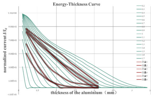
Figure 8: The actual energy-thickness curves compared with the simulation result.
