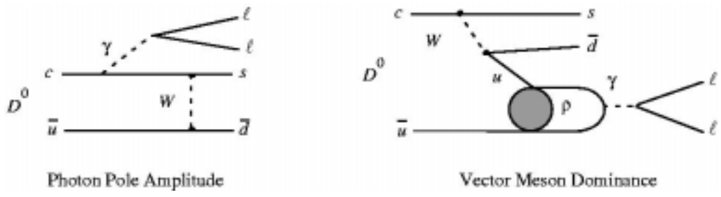
Figure 2.1: Photon Pole Amplitude and Vector Meson Dominance.
