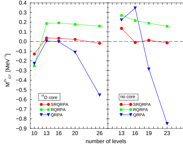
Fig. 1. Dependence of the ^{76}\text{Ge} \rightarrow ^{76}\text{Se} two-neutrino nuclear matrix elements M^{2\nu} on the dimension of the single-particle basis within the QRPA, the RQRPA and the SRQRPA.
