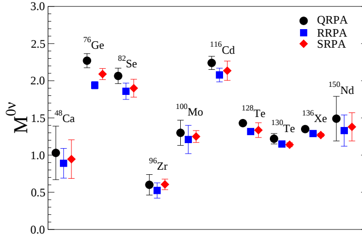
Fig. 2. Average neutrinoless nuclear matrix elements M^{0\nu} and their variance within the QRPA, the RQRPA and the SRQRPA.
