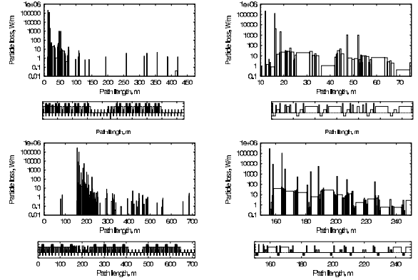
FIGURE 3. Beam loss in PD-II at 8 GeV (top) and PD-I at 16 GeV (bottom).
