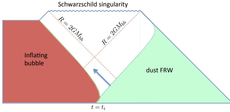
Figure 3. Formation of a black hole by a large vacuum bubble, with M_{\text{bh}} \gg M_{\text{cr}} , in a dust dominated spatially flat FRW. In this case, the bubble does not collapse into the Schwarzschild singularity. Instead, at the time t_{\text{cr}} \sim \text{Min}\{t_{\text{b}}, t_{\sigma}\} the size of the bubble starts growing exponentially in a baby universe, which is connected by a wormhole to the parent dust dominated FRW universe. Initially, a geodesic observer at the edge of the dust region can send signals through the wormhole into the baby universe. This is represented by the blue arrow in the figure. However, after a proper time t \sim 2GM_{\text{bh}} , the wormhole “closes” and any signals which are sent radially inwards end up at the Schwarzschild singularity.
