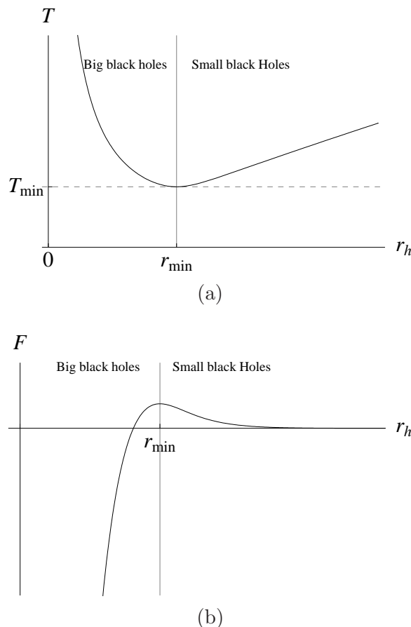
Figure 1. Typical plots of the black-hole temperature (a) and free energy (b) as a function of the horizon position r_h , in a confining background. The temperature features a minimum at r_{\min} , that separates the large black-hole from the small black-hole branches.
