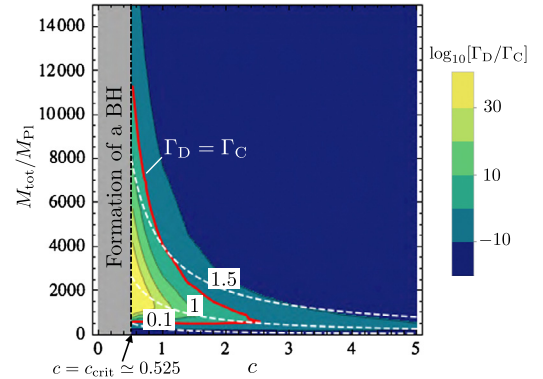
Fig. 3. A plot of the ratio of the decay rate, \Gamma_D , to the inverse of the cosmological time, \Gamma_C , as a function of the mass and compactness of the horizonless object. The contour of \Gamma_D = \Gamma_C (red solid line) and contours of \xi/R_{\text{CDL}} (white dashed lines) are marked for reference. In the case of c \leq c_{\text{crit}} \simeq 0.525 (gray shaded region), the object inevitably collapses to a BH since a function f_+(r) has zero points there.
