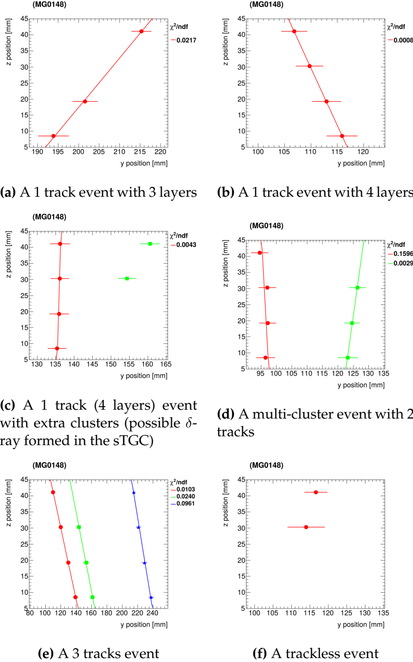
Figure 5.1: Different categories of cosmic ray events, based on their tracking. Note the z-axis is defined to be the direction of the muon flight (from the ceiling to the ground). The first layer of the sTGC quadruplet is at 8.1mm and the fourth layer is at 41.1mm.
