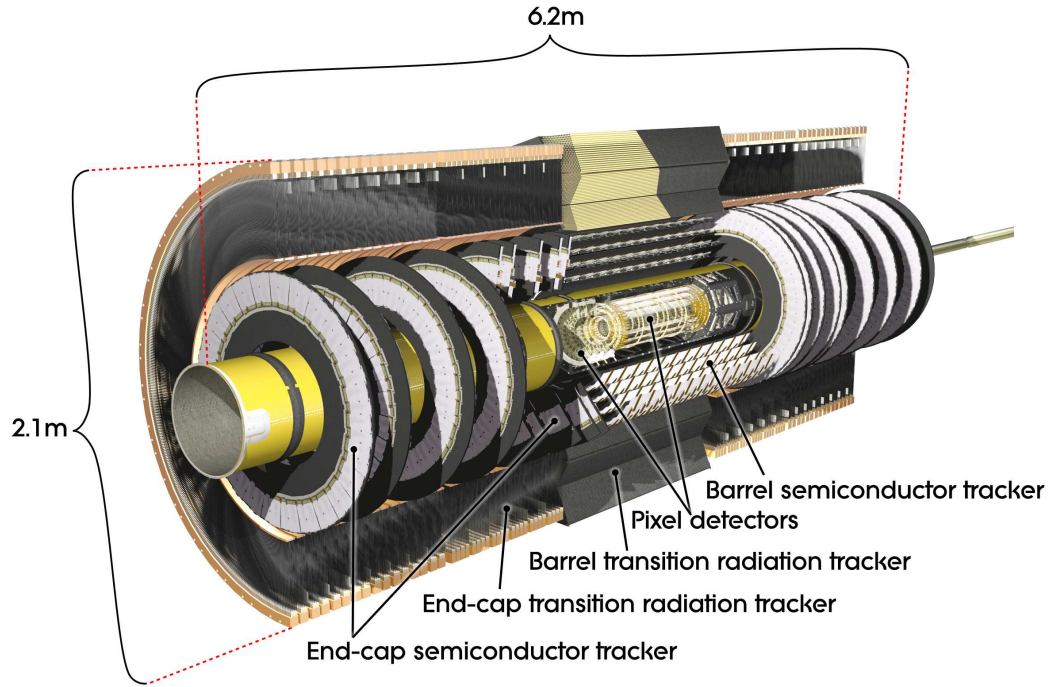
Figure 3.3: Illustration of the ATLAS inner detector.
