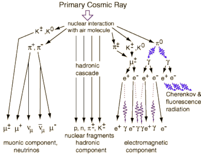
Figure 2.2: The secondary particles of a cosmic ray decay, resulting from the interaction with nuclei from atmospheric atoms [23]. Pions and kaons usually decay muonically [14].
