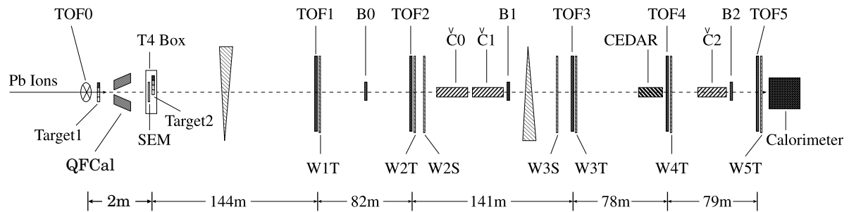
Figure 1. The NA52 experimental set-up.
