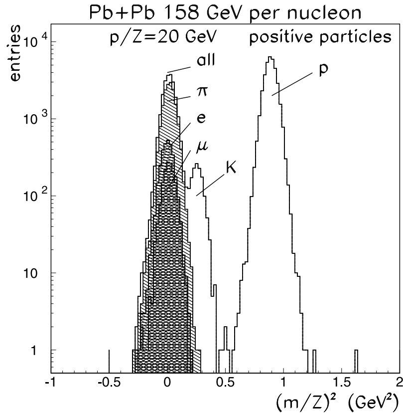
Figure 5. Typical example of particle identification at p/Z = 20 GeV/c. K^+ , p and heavier particles are separated using TOF information, while \pi^+ , \mu^+ and e^+ are identified using calorimeter and Čerenkov information.
