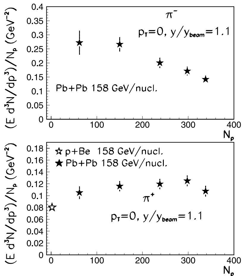
Figure 10. Charged pion invariant yields in Pb + Pb collisions at 158 A GeV near zero p_T divided by the mean number of participating nucleons in the reaction ( N_p ) as a function of N_p at a rapidity of 6.3. The p + Be data were measured at 450 GeV/nucleon in the same p_T and y/y_{\text{beam}} [14] and have been rescaled to 158 A GeV (see text).
