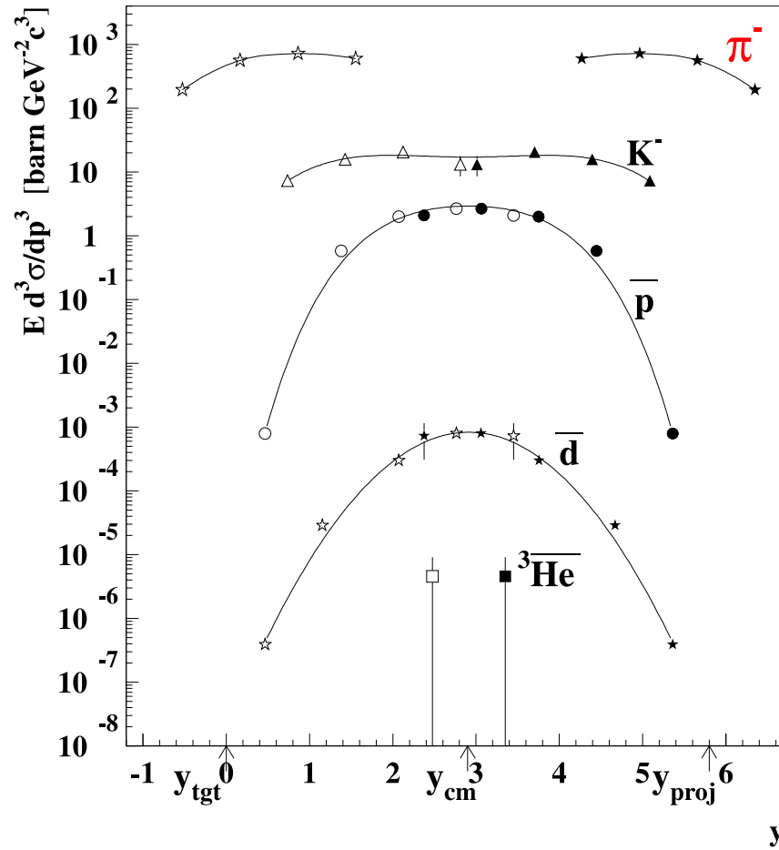
Figure 7. Invariant production cross sections of negative particles and antinuclei in minimum-bias Pb + Pb collisions at 158 A GeV near zero p_T . Full symbols refer to the measured points; the open symbols are points reflected over midrapidity ( y_{cm} = 2.9 ). The curves are drawn to guide the eye.
