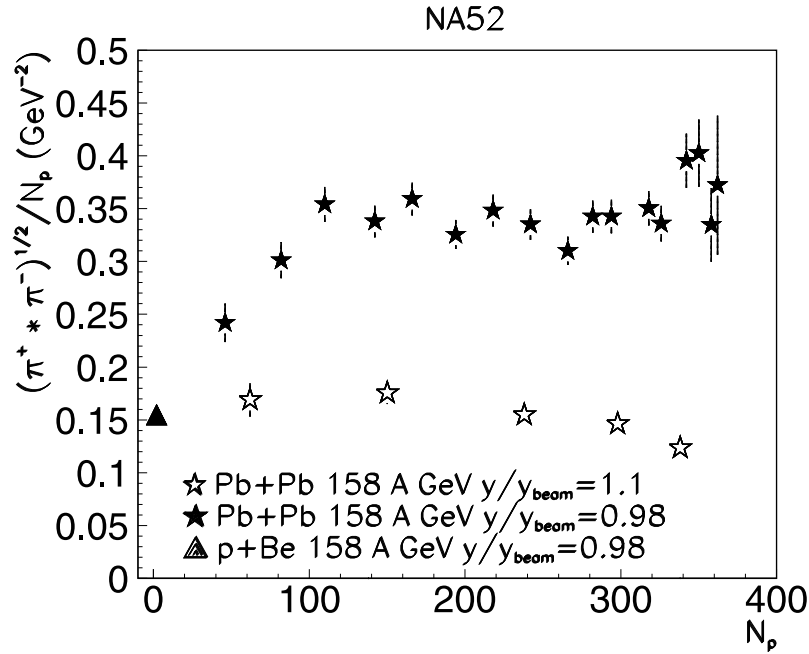
Figure 13. Square root of the product of the invariant differential yields ( E d^3N/d^3p ) of the positive pions times those of the negative pions at y = 5.7 and 6.3 divided by the mean total number of participating nucleons N_p as a function of N_p near zero p_T . NA52 data from Pb + Pb collisions at 158 A GeV are compared with p + Be collisions measured at 450 GeV/nucleon [14], which were rescaled to 158 GeV/nucleon at similar p_T and y/y_{\text{beam}} \sim 0.97 ( y = 5.7 in Pb + Pb).
