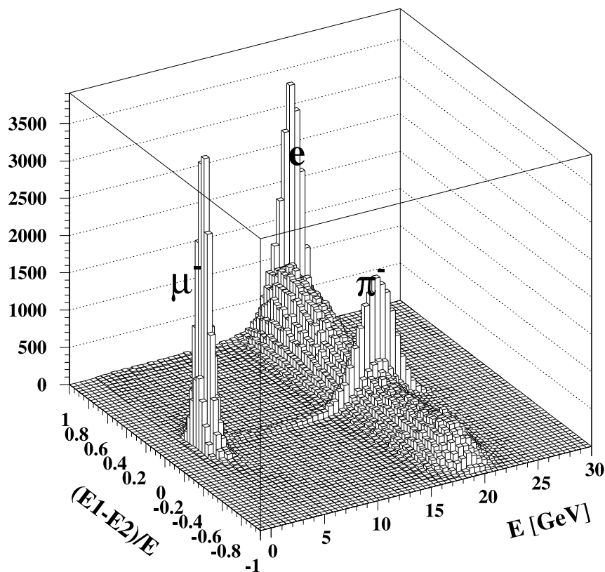
Figure 4. Difference of the energy deposited in the first and second hadronic calorimeter module (E1 - E2) over the total energy deposited in the calorimeter E , displayed as a function of the latter, for negative particles with p/Z = 20 GeV.
