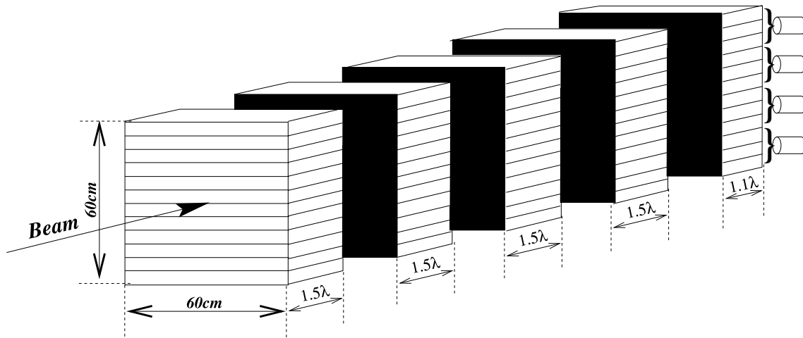
Figure 2. The hadronic calorimeter.
