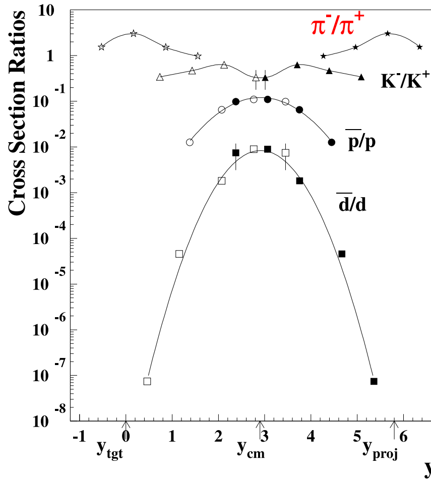
Figure 8. Rapidity dependence of particle cross section ratios in minimum-bias Pb+Pb collisions at 158 A GeV near zero p_T . Full symbols refer to the measured points; the open symbols are points reflected over midrapidity ( y_{cm} = 2.9 ). The curves are drawn to guide the eye.
