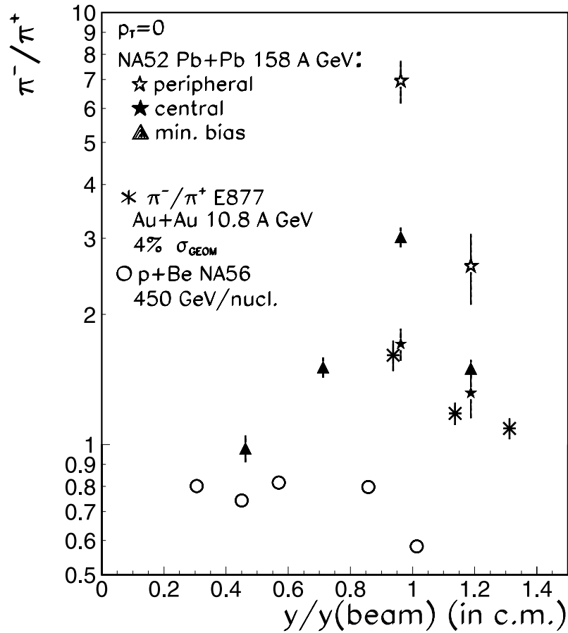
Figure 12. \pi^-/\pi^+ ratio near zero p_T as a function of rapidity normalized to the beam rapidity in the c.m. system. NA52 data from peripheral, central and minimum-bias Pb + Pb collisions at 158 A GeV are shown and compared with central Au + Au collisions at 10.8 GeV/nucleon [18] and with p + Be reactions at 450 GeV/nucleon [14].
