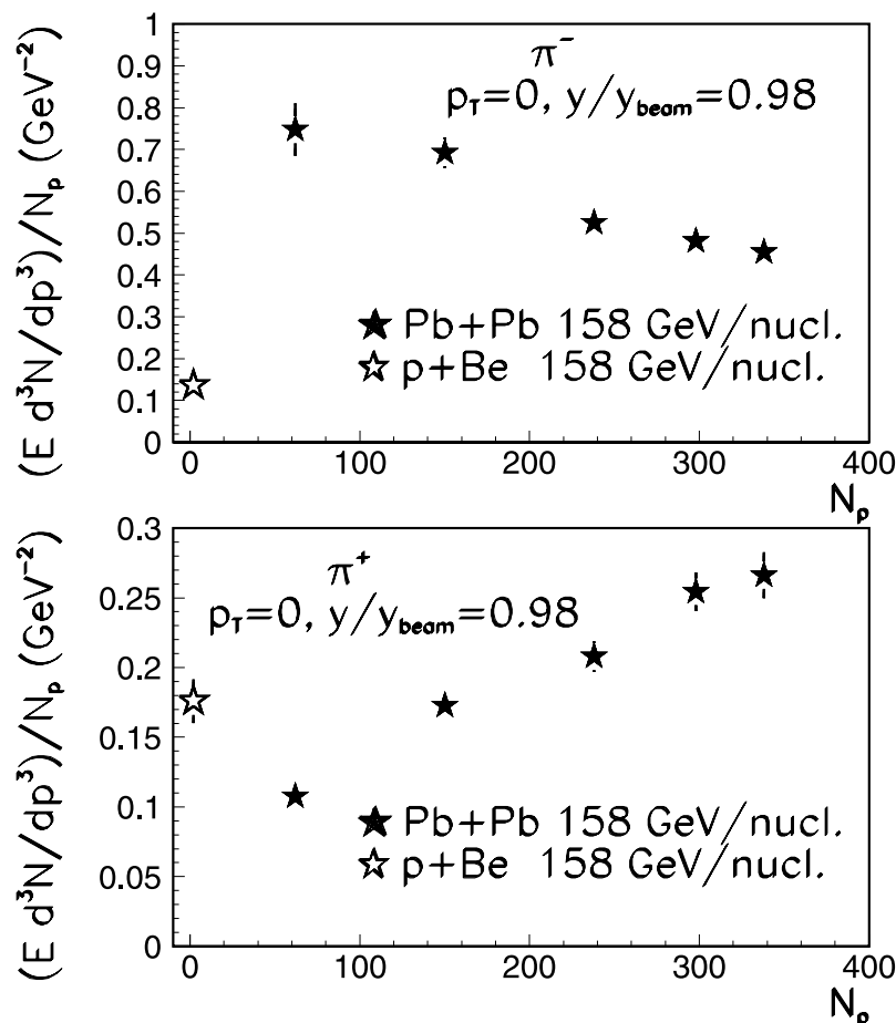
Figure 9. Charged pion invariant yields in Pb + Pb collisions at 158 A GeV near zero p_T divided by the mean number of participating nucleons in the reaction ( N_p ) as a function of N_p at a rapidity of 5.7. The p + Be data were measured at 450 GeV/nucleon at the same p_T and y/y_{\text{beam}} [14] and have been rescaled to 158 A GeV (see text).
