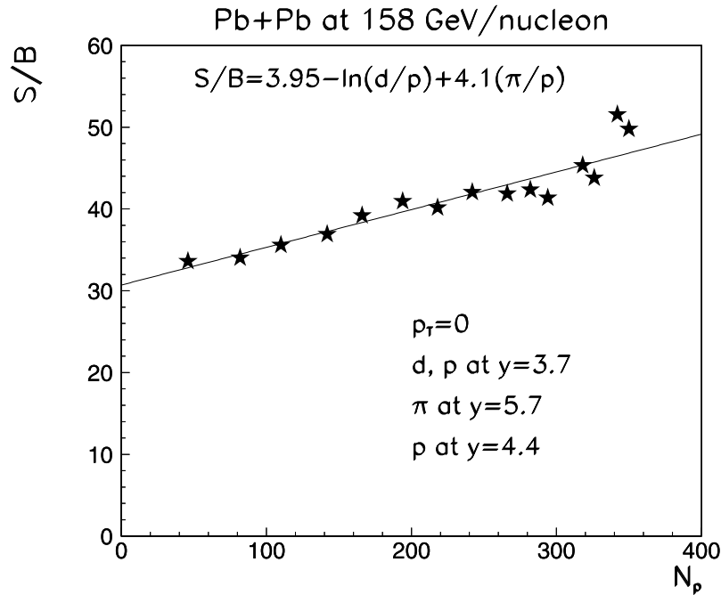
Figure 14. Entropy per baryon ( S/B ) as a function of the number of participants in Pb + Pb collisions at 158 A GeV. (See text for explanations.)
