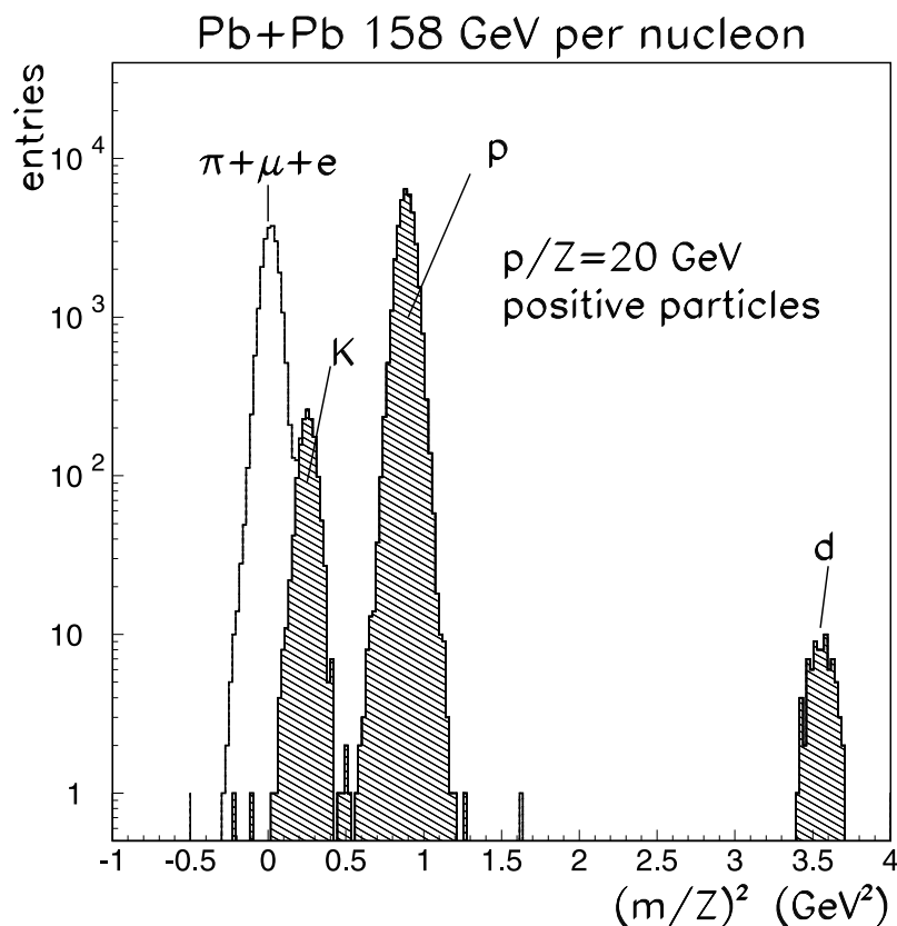
Figure 3. Typical example of a (m/Z)^2 spectrum of positive particles obtained from time-of-flight measurements at p/Z = 20 GeV. The shaded area indicates particles which gave no light in the Čerenkov counter.
