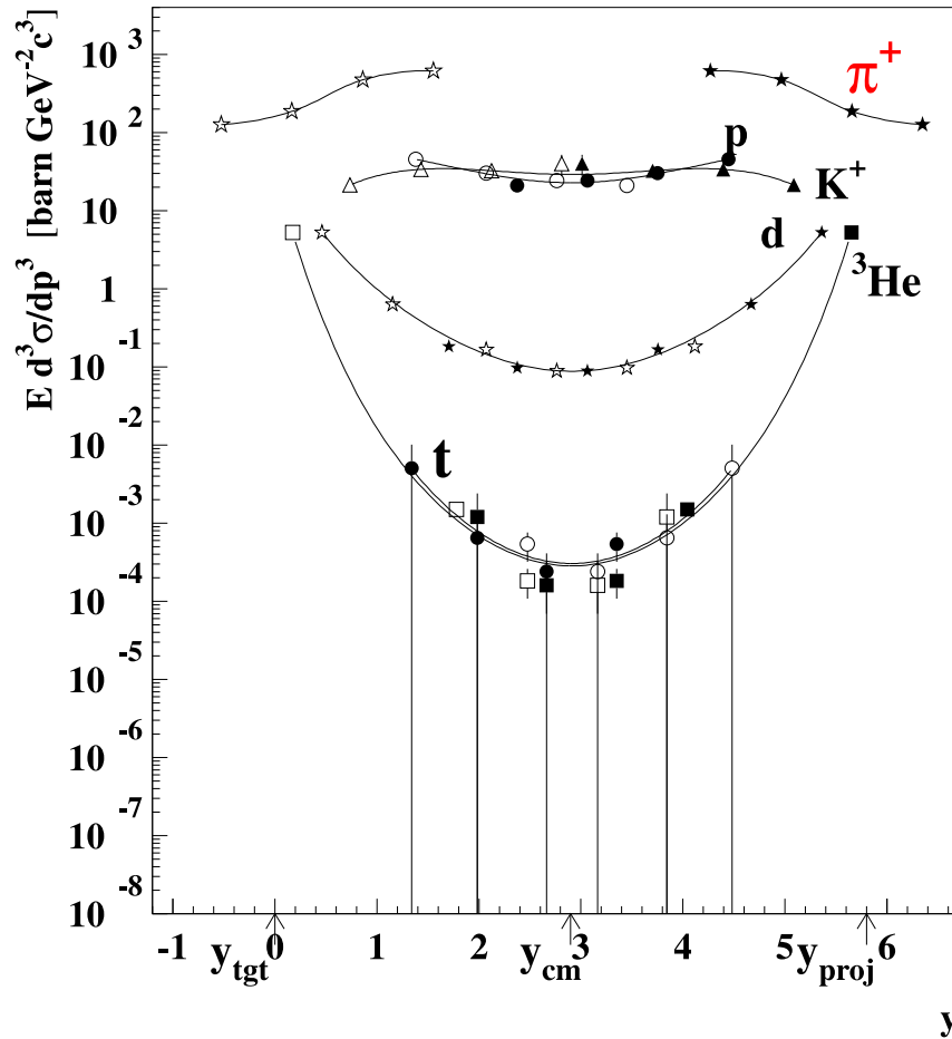
Figure 6. Invariant production cross sections of positive particles and nuclei in minimum-bias Pb + Pb collisions at 158 A GeV near zero p_T . Full symbols refer to the measured points; the open symbols are points reflected over midrapidity ( y_{cm} = 2.9 ). The curves are drawn to guide the eye.
