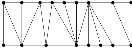
Fig. 2. The propagation of a spatial slice from time t to time t + 1 . The ends of the strip should be joined to form a band with topology S^1 \times [0, 1] .
