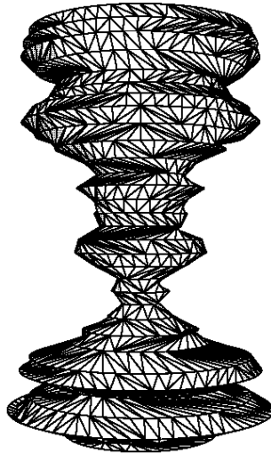
Fig. 1. Piecewise linear space-time histories 1+1 dimensional quantum gravity.
