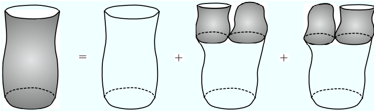
Fig. 3. In all four graphs, the geodesic distance from the final to the initial loop is given by t . Differentiating with respect to t leads to Eq. (20). Shaded parts of graphs represent the full, g_s -dependent propagator and disc amplitude, and non-shaded parts the CDT propagator.
