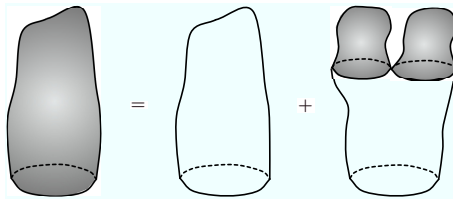
Fig. 4. Graphical illustration of Eq. (65). Shaded parts represent the full disc amplitude, unshaded parts the CDT disc amplitude and the CDT propagator.
