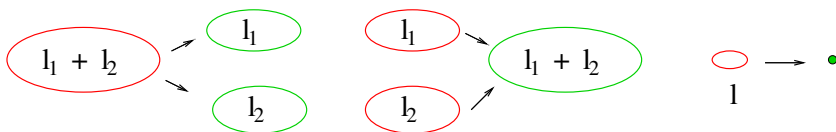
Fig. 5. Graphical illustration of the various terms in Eq. (45).
