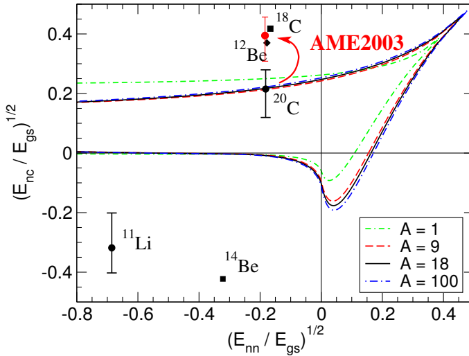
Fig. 6. Boundary curves for the existence of an excited Efimov state as function of the neutron–core energy E_{nc} and neutron–neutron energy E_{nn} in units of the three-body ground state energy E_{gs} . The shift of ^{20}\text{C} from using the values of the newer AME2003 atomic mass evaluation [21] is indicated by the arrow.
