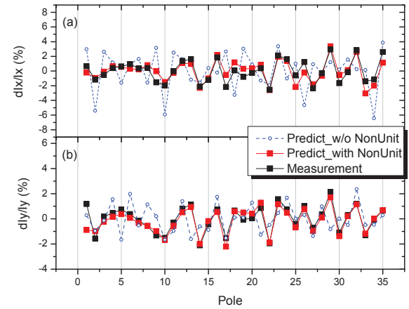
Figure 4: Distribution of deviation of first field integral of poles: (a) horizontal field; (b) vertical field.
