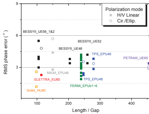
Figure 6: Map of r.m.s. phase error of APPLE-II EPU in several facilities.
