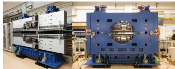
Figure 1: The front side of EPU48 is shown at the left, the rear side at the right.
