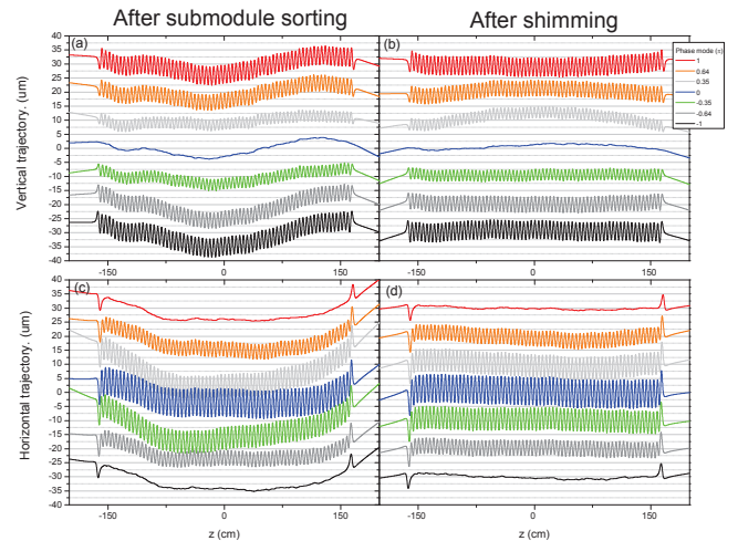
Figure 5: Straightness of (a,b) vertical and (c,d) horizontal trajectories; (a,c) before shimming, (b,d) after shimming.
