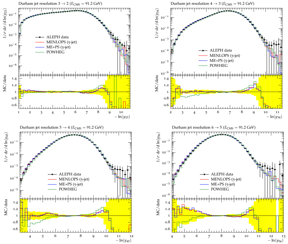
Figure 3.21: Durham d_{n \rightarrow n+1} jet resolutions at LEP compared to data taken by the ALEPH experiment [112].
