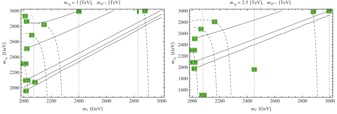
Fig. 2. Contour plots for the masses of DCHs as functions of m_{A_1} and m_V . The left (right) panel corresponds to m_{A_2} = 1 (2.5) TeV. The heaviest DCH is represented by dotted curves, the second heaviest by dashed curves, and the lightest by solid curves.
