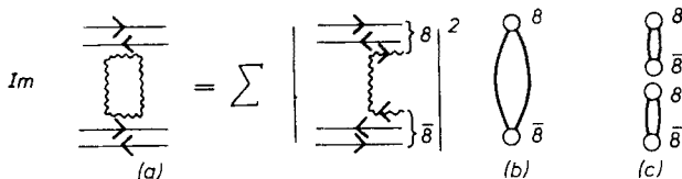
Fig. 10. a) the s -channel structure of diagram 9b, b) system of octet-anti-octet joined with two (3, \bar{3}) chains, and c) a colour structure for diffractive excitations
