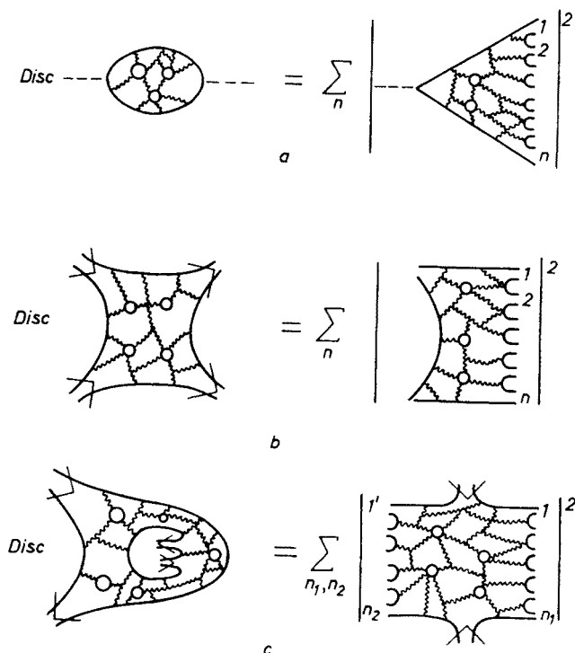
Fig. 6. a) 1/n expansion for \sigma_{\text{tot}}(e^+e^- \rightarrow \text{hadrons}) ; b) s -channel content of the bare reggeon; c) s -channel content of the bare Pomeron
