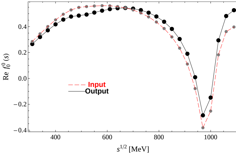
Fig. 3. \text{Re} f_0^0(s) for input and output before fitting.
