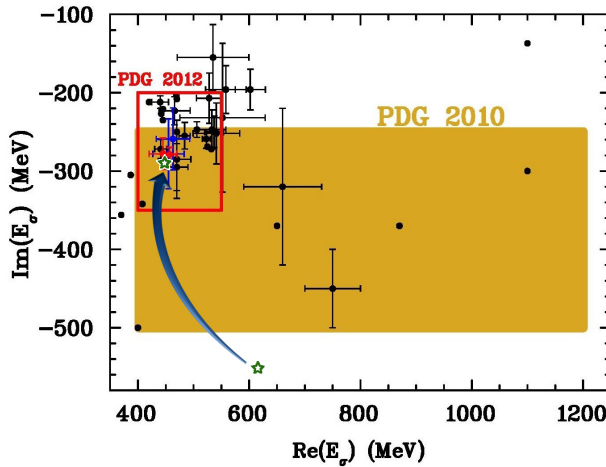
Fig. 5. Movement of the \sigma pole due to the fit to the GKPY equations.
