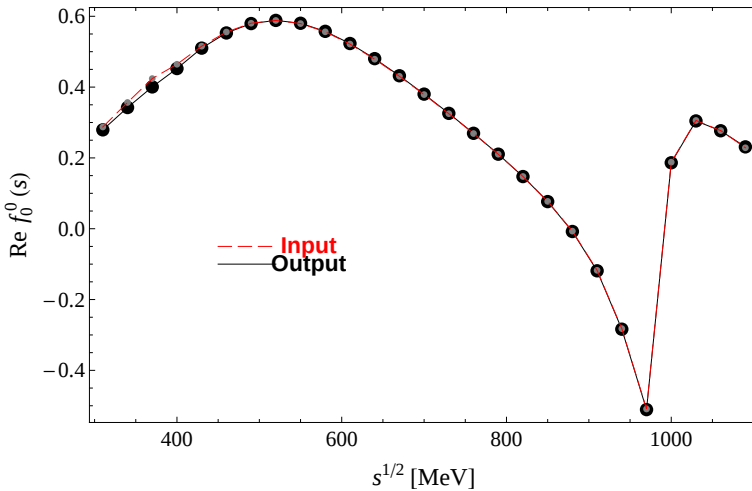
Fig. 4. \text{Re} f_0^0(s) for input and output after fitting.
