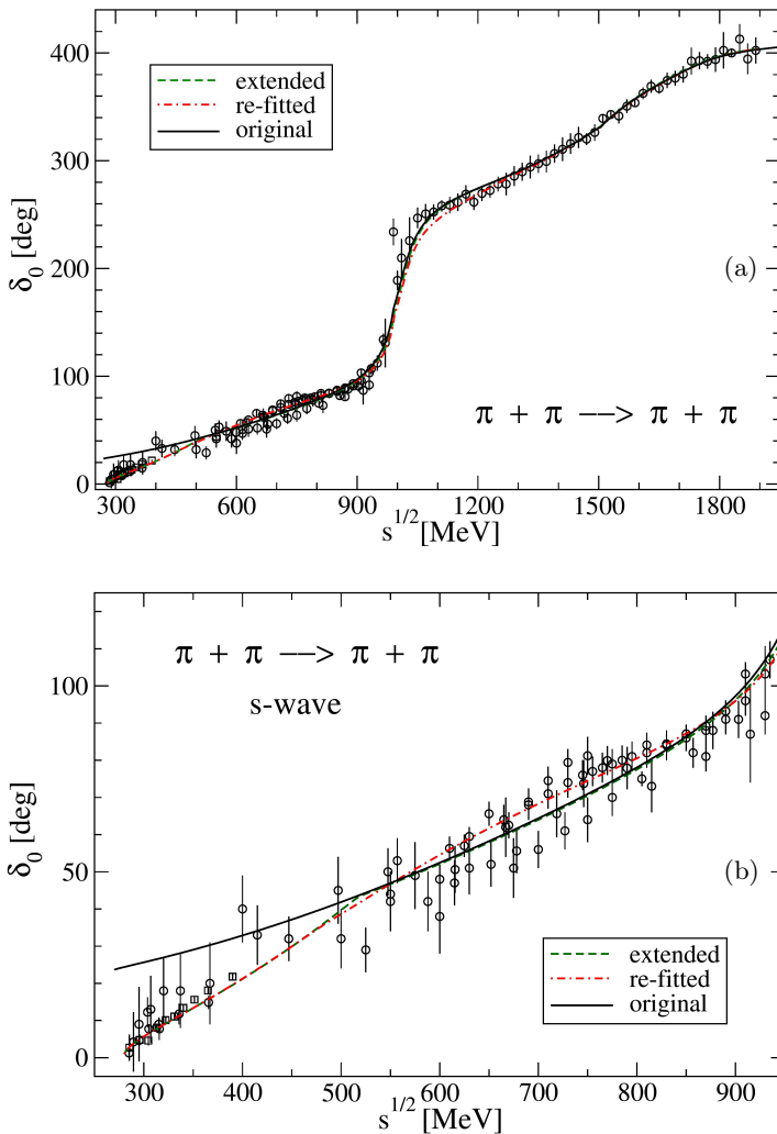
Fig. 2. Phase shift versus energy for S-wave.
