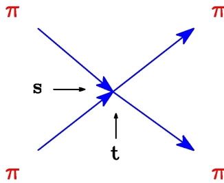
Fig. 1. Crossing symmetry.
