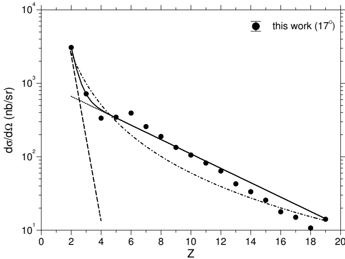
Fig. 16. (Colour on-line) The energy-integrated cross sections at \vartheta = 17^\circ as a function of the fragment charge number Z . A fit with two exponentials is also shown (solid curve). The two components are also shown separately: the small charge component as long-dashed curve, the one for heavier charges as dotted curve. The dash-dotted curve indicates a power law fit.
