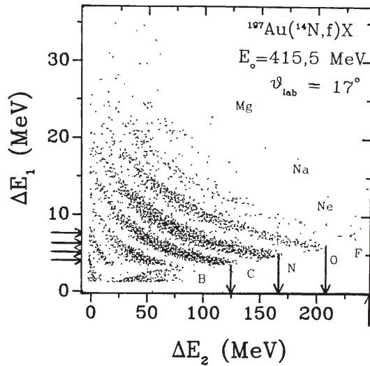
Fig. 3. The response of the ionisation chamber ( \Delta E_1 ) versus the first silicon counter ( \Delta E_2 ) as a scatter plot from a nitrogen beam hitting on the gold target. The arrows indicate the energies deposited in the counters for the particles stopped with maximal energy in the silicon counter. The different elements are indicated next to the appropriate hyperbola.
