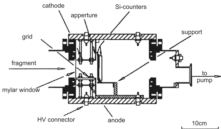
Fig. 2. Layout of the ionisation chamber.
