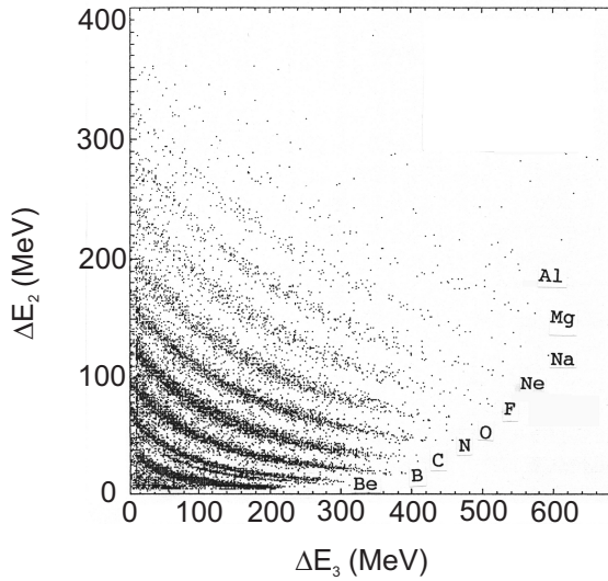
Fig. 5. The same as Fig. 4 but for \Delta E_2 - \Delta E_3 plot measured with two silicon counters.
