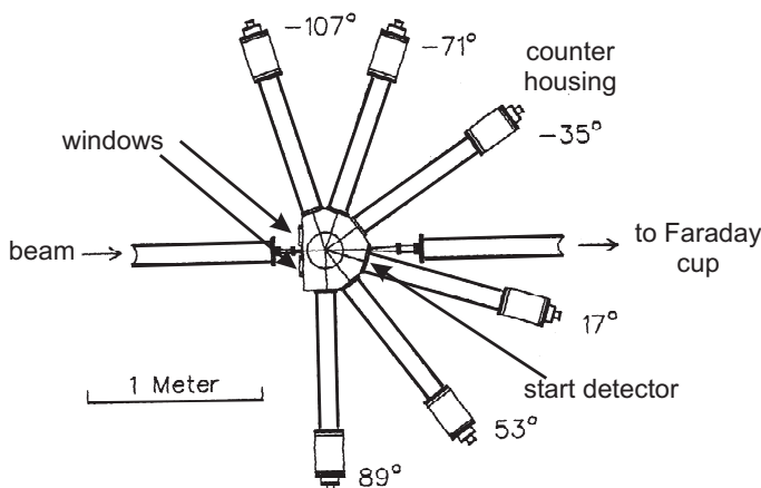
Fig. 1. Layout of the reaction chamber. The boxes at the ends of tubes house the counters. For the measurements at large angles, the tubes were removed to enlarge the solid angle (see Table I).
