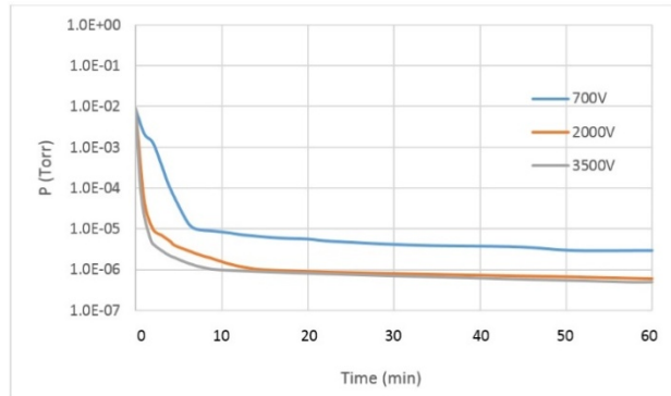
Figure 4: Pressure versus Time for 700, 2000 and 3500 volt anode voltages.
