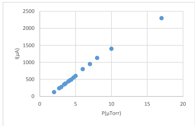
Figure 5: Penning discharge current dependency versus pressure.
