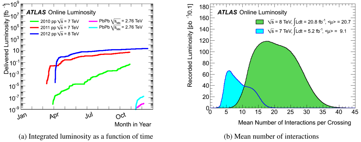
Figure 3.2: Performance of the LHC. (a) The cumulative luminosity delivered by the LHC in 2010, 2011 and 2012. The last months of each running period were devoted to collisions of lead-ions. (b) The luminosity-weighted distribution of the mean number of interactions per bunch crossing for the 2011 (light blue shaded area) and 2012 (dark green shaded area) pp data.
