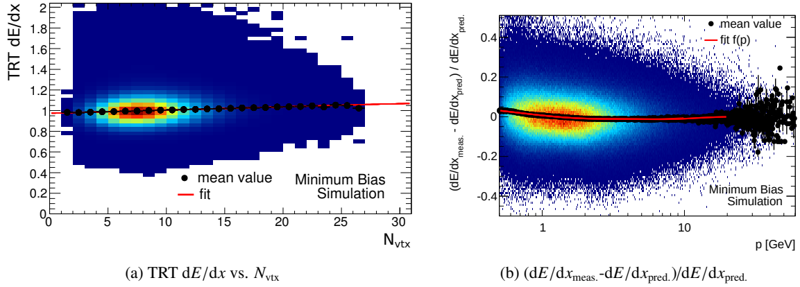
Figure 5.12: (a) TRT dE/dx plotted as a function of the number of primary vertices in the Minimum Bias Monte Carlo sample. Overlaid is the profile distribution (black points) and the linear fit to the profile (red) [90]. (b) The dependence of the relative difference between the predicted ( dE/dx_{\text{pred.}} ) and measured dE/dx ( dE/dx_{\text{meas.}} ) on track momentum in the Minimum Bias Monte Carlo sample. The black dots represent the mean value in each momentum bin, whereas the red line is the fit on which the momentum correction is based [90].
