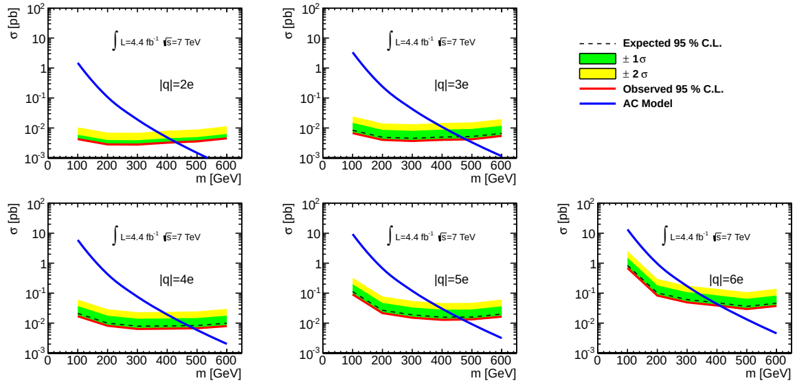
Figure 8.3: 95% CL limits on the production cross section of multi-charged highly-ionizing particles. The black dotted line shows the expected limit and the \pm 1\sigma (green) and \pm 2\sigma (yellow) uncertainty bands. The observed limit (red) is compared with the predicted cross section from the almost commutative (AC) model. The plots are shown separately for charges |q| = 2e to |q| = 6e .
