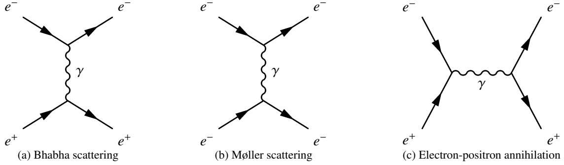
Figure 4.1: The processes contributing to the energy loss of electrons and positrons in matter.
