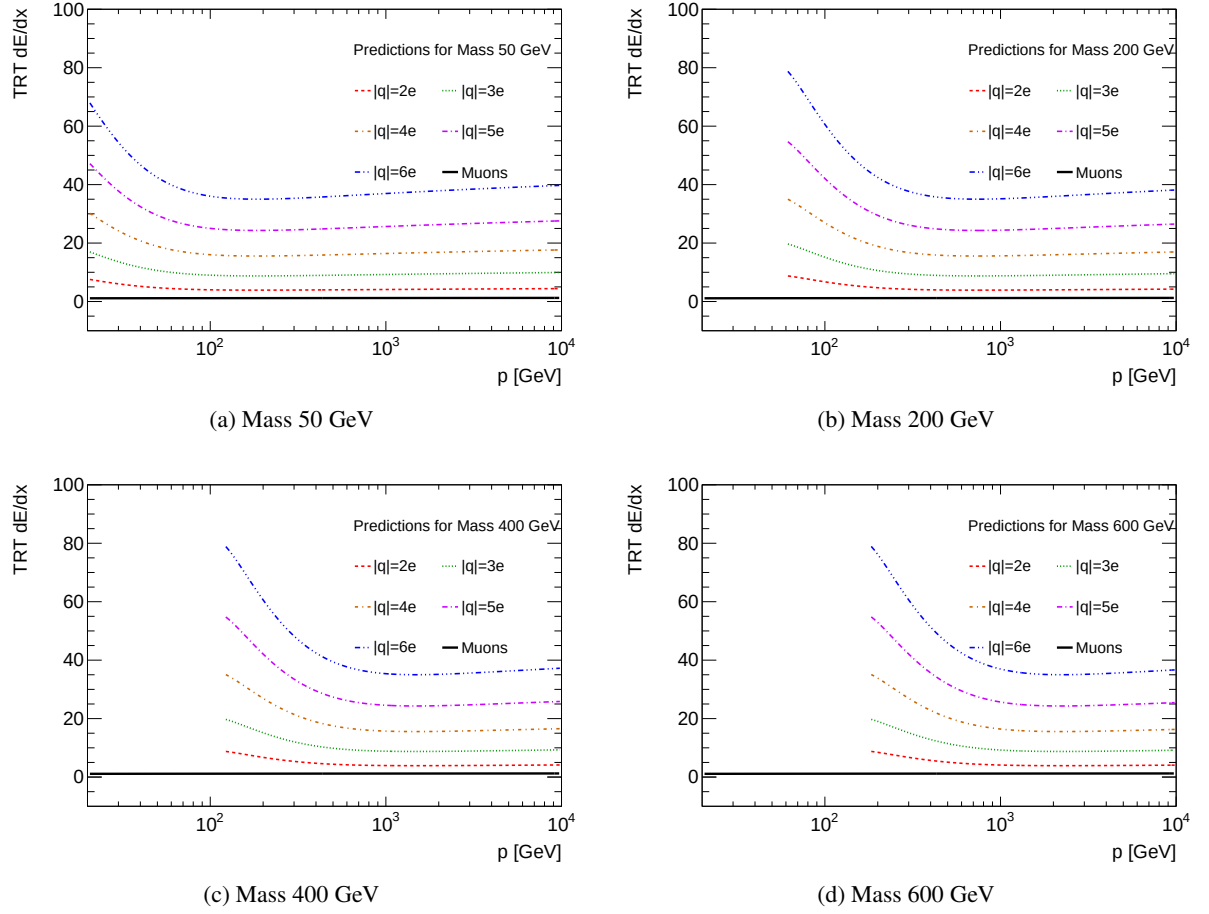
Figure 5.20: The predicted TRT dE/dx for multi-charged particles and muons as extrapolated from the fit to |q| = 1e particles versus the true particle momentum p for masses 50 GeV (a), 200 GeV (b), 400 GeV (c) and 600 GeV (d). The validity range of the dE/dx fit above \beta\gamma = 0.5 translates into a cut-off at lower momentum values p = 0.5m for a given mass m .
