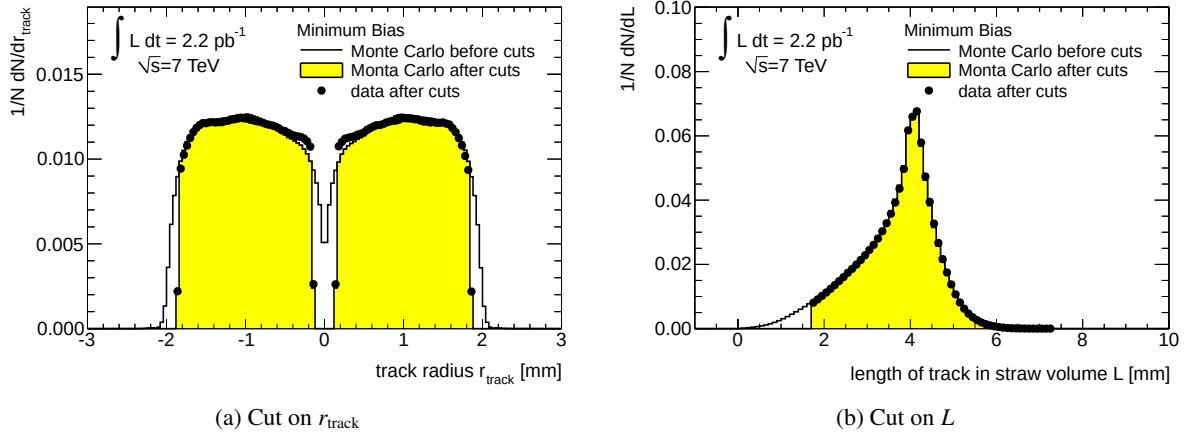
Figure 5.7: The distribution of hits as a function of (a) r_{\text{track}} and (b) L before the cut (solid black line) and after the cut (shaded yellow area) on these variables. The plots show distributions from the Minimum Bias Monte Carlo and data samples [90].
