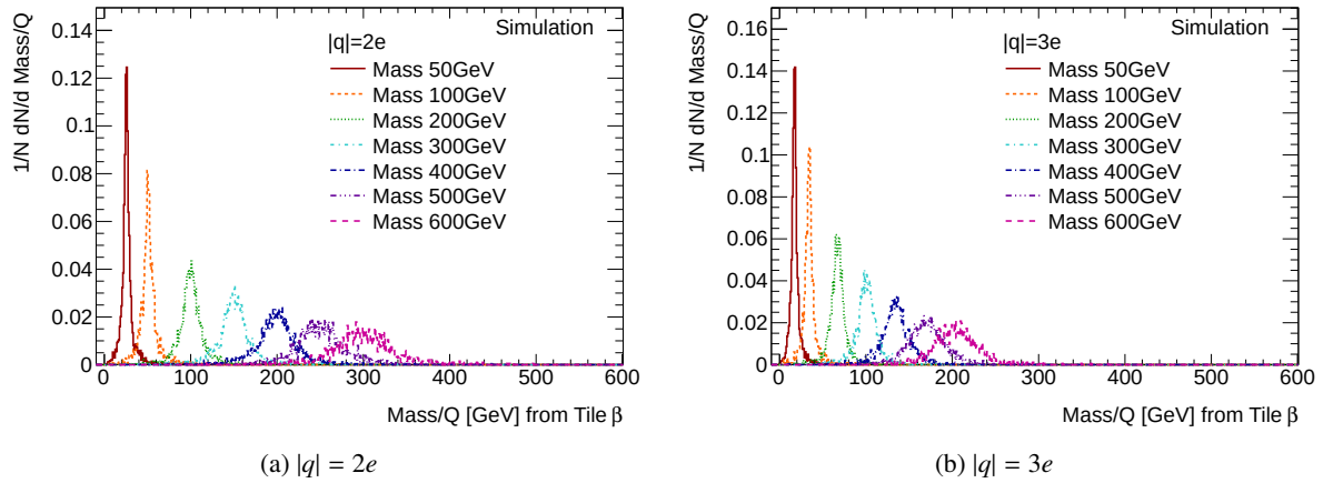
Figure 6.13: The mass/ |q| measurement extracted from \beta_{\text{Tile}} exemplary for signals with charge |q| = 2e (a) and |q| = 3e (b).
