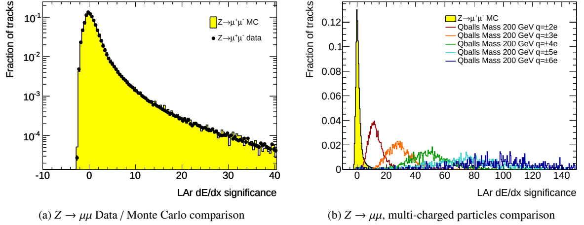
Figure 6.12: Normalized distribution of S(\text{LAr } dE/dx) in the direct data / Monte Carlo comparison of Z \rightarrow \mu\mu events (a) and for simulated muons and multi-charged particles (b). In the latter the distributions are shown for the signal samples of charge |q| = 2 - 6e and mass 200 GeV [82] (see also [38]).
