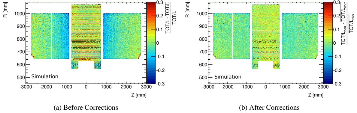
Figure 5.5: Relative deviation of ToT/L from the mean value shown in the r - z -plane before (a) and after (b) the corrections in r_{\text{drift}} and s [90].
