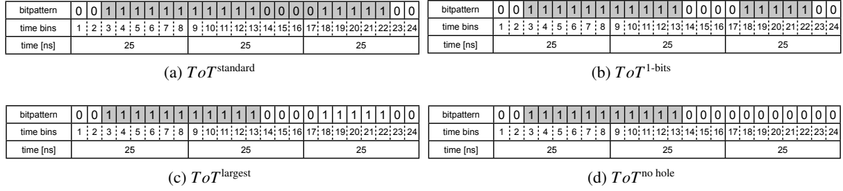
Figure 5.3: The four different definitions of a ToT from the TRT bitpattern considered in this thesis.
