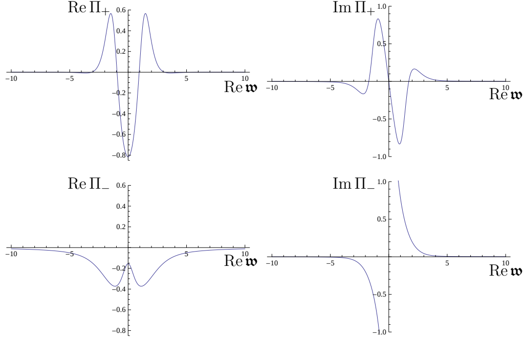
Fig. 2.5: Slices through the (\text{Re } w, q) plane of \Pi_+ (top row) and \Pi_- (bottom row) at q = 10^{-6} and T/\mu = 0.09 . The left and right panels show the real and imaginary parts, respectively.
