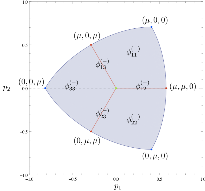
Fig. 5.4: Modes which give the highest critical temperature. The diagonal modes \phi_{11}^{(-)}, \phi_{22}^{(-)}, \phi_{33}^{(-)} give the highest critical temperature in the blue regions as shown. In addition, along the red lines the modes \phi_{12}^{(-)}, \phi_{13}^{(-)}, \phi_{23}^{(-)} linearly coincide with the diagonal modes and have the same critical temperature. Dots indicate special cases of the chemical potentials, (\mu_1, \mu_2, \mu_3) , with all equal at the origin.
