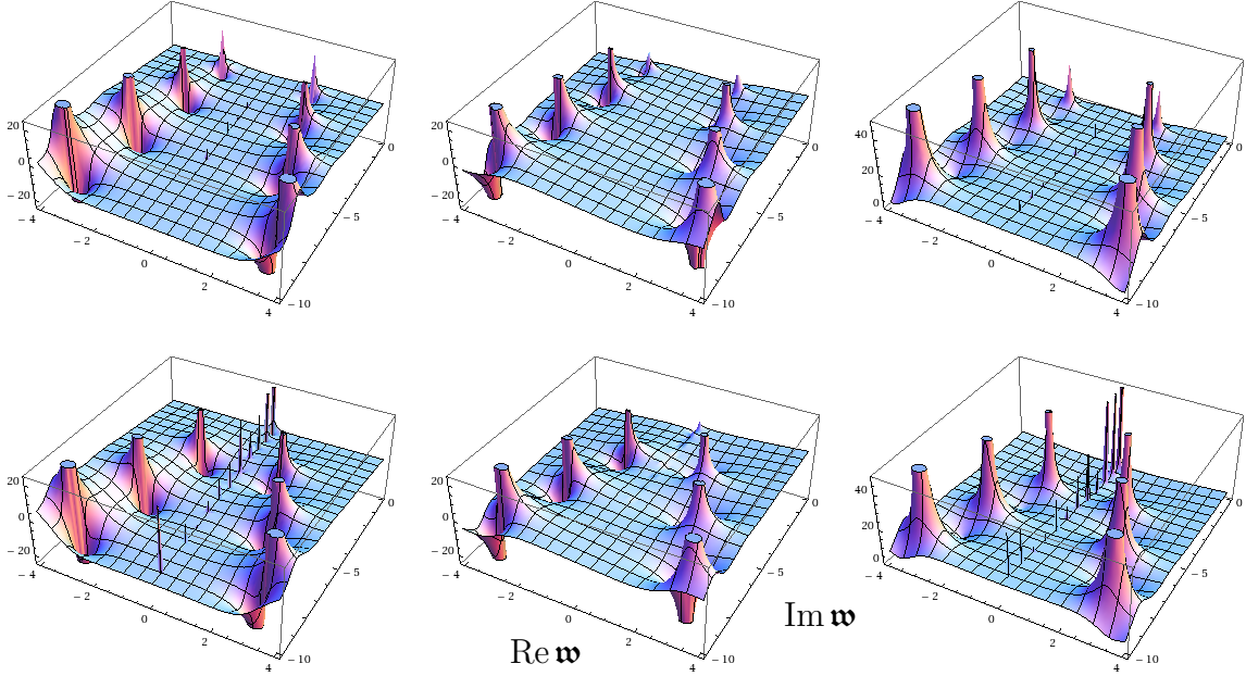
Fig. 2.3: Surface plots of \Pi_+ (top row) and \Pi_- (bottom row) on the complex w plane at q = 1 , T/\mu = 0.09 . We show (from left to right) the real part, imaginary part and absolute value of each. All plots have the same orientation on the plane, as indicated.
