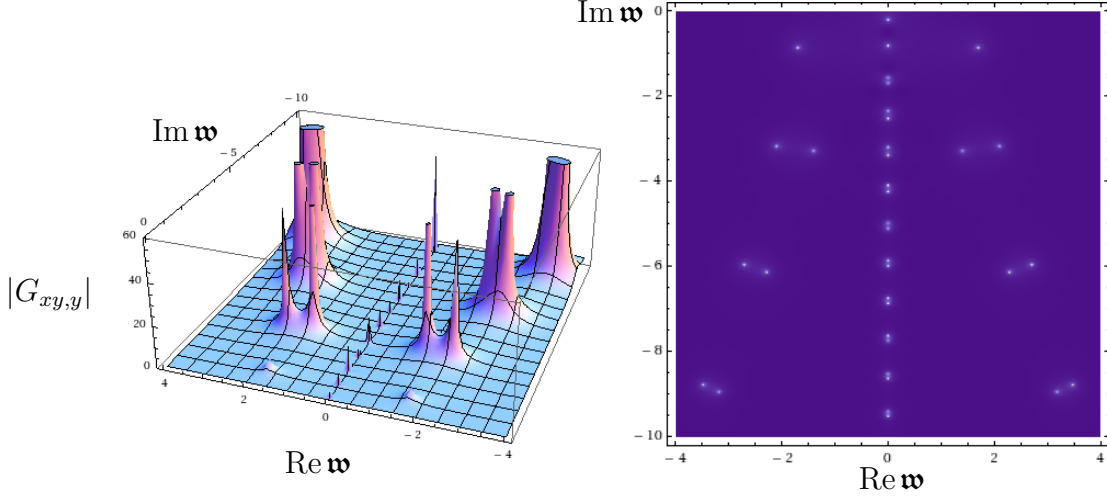
Fig. 2.2: A comparison between a surface plot of |G_{xy,y}| on the complex w plane (left) and the appropriate quasinormal frequencies (right). Both plots have q = 1 and T/\mu = 0.09 .
