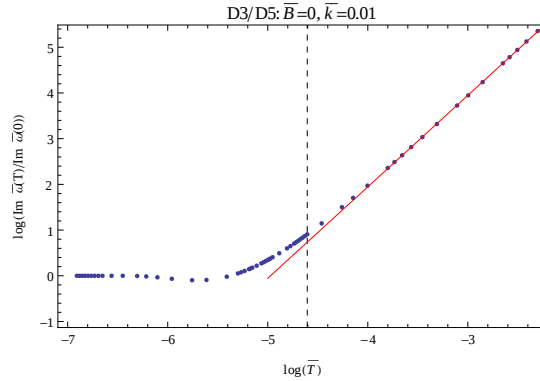
Fig. 3.3: Logarithm of the decay rate of the holographic zero sound mode in the D3/D5 system at B = 0 , normalised to the T = 0 value, \log(\text{Im} \bar{\omega}(\bar{T})/\text{Im} \bar{\omega}(0)) , as a function of \log \bar{T} for \bar{k} = 0.01 , within the regime \bar{T}^2 \ll \bar{k} . The dots are our numerical results, the vertical dashed black line denotes \bar{T} = \bar{k} , and the solid red best-fit line has gradient 2, indicating that \text{Im} \bar{\omega}(\bar{k}) \propto \bar{T}^2 for \bar{T} \gtrsim \bar{k} .
