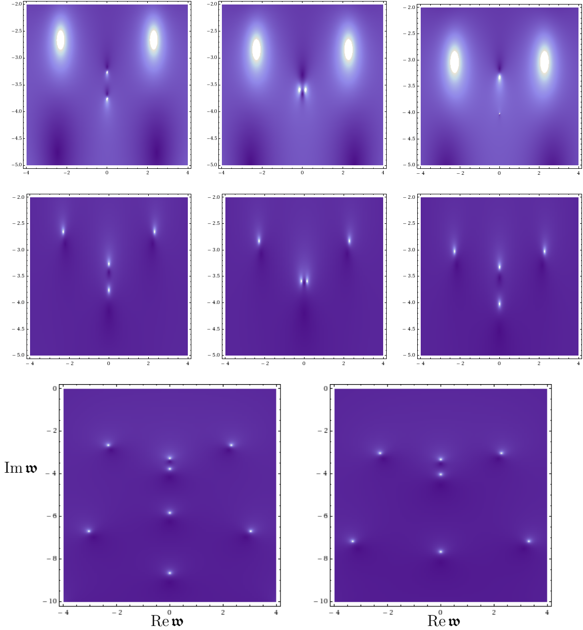
Fig. 2.8: Density plots of |\Pi_-| on the complex \mathfrak{w} plane at fixed \mathfrak{q} = 3 are shown in the upper row. The values of T/\mu are (from left to right) 0.185, 0.2 and 0.215. These plots have been cropped to include only the poles which move off-axis and the leading poles. For comparison, the quasinormal frequencies at the same values of parameters are given in the second row. The final row contains two quasinormal frequency plots, one at T/\mu = 0.185 and one at T/\mu = 0.215 . These show a larger region of the complex \mathfrak{w} plane, including the origin, for orientation.
