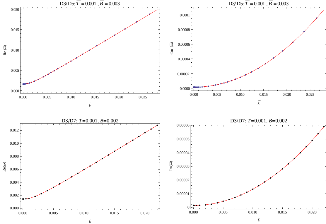
Fig. 3.8: Top: \text{Re} \bar{\omega}(\bar{k}) (left) and -\text{Im} \bar{\omega}(\bar{k}) (right) versus \bar{k} for the holographic zero sound mode in the D3/D5 system with \bar{B} = 0.003 and \bar{T} = 0.001 , in the range \bar{k} \gg \bar{T} . Bottom: \text{Re} \bar{\omega}(\bar{k}) (left) and -\text{Im} \bar{\omega}(\bar{k}) (right) versus \bar{k} for the holographic zero sound mode in the D3/D7 system with \bar{B} = 0.002 and \bar{T} = 0.001 , in the range \bar{k} \gg \bar{T} . In all four plots the dots are our numerical results and the solid red lines come from the T = 0 dispersion relation, (3.42). Clearly the T = 0 result (3.42) is a very good approximation to the low-temperature dispersion relation, as was the case when B = 0 (recall fig. 3.2).
