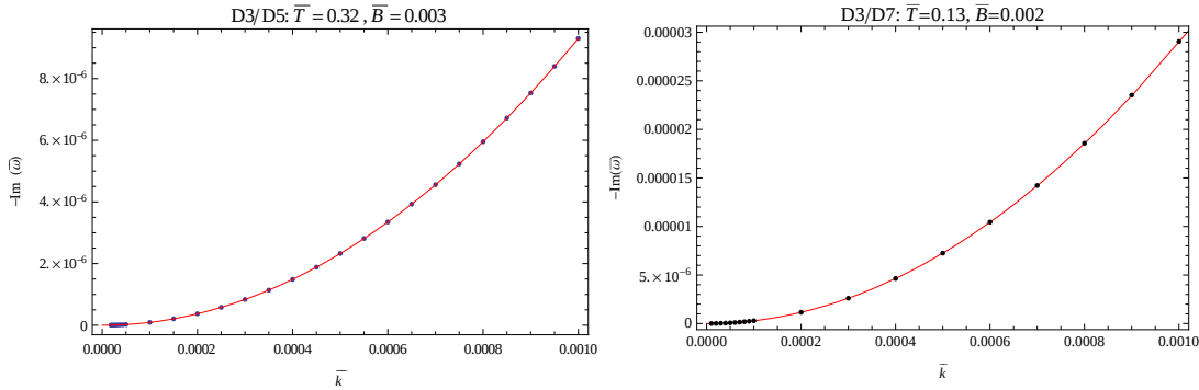
Fig. 3.9: Left: -\text{Im } \bar{\omega} versus \bar{k} for the charge diffusion mode in the D3/D5 system with \bar{B} = 0.003 and \bar{T} = 0.32 , within the range \bar{k} \ll \bar{T}^2 . Right: The same for the D3/D7 system, with \bar{B} = 0.002 and \bar{T} = 0.13 . For both modes, \text{Re } (\bar{\omega}) = 0 . In both plots the dots are our numerical results and the solid red lines are the dispersion relation in (3.49).
