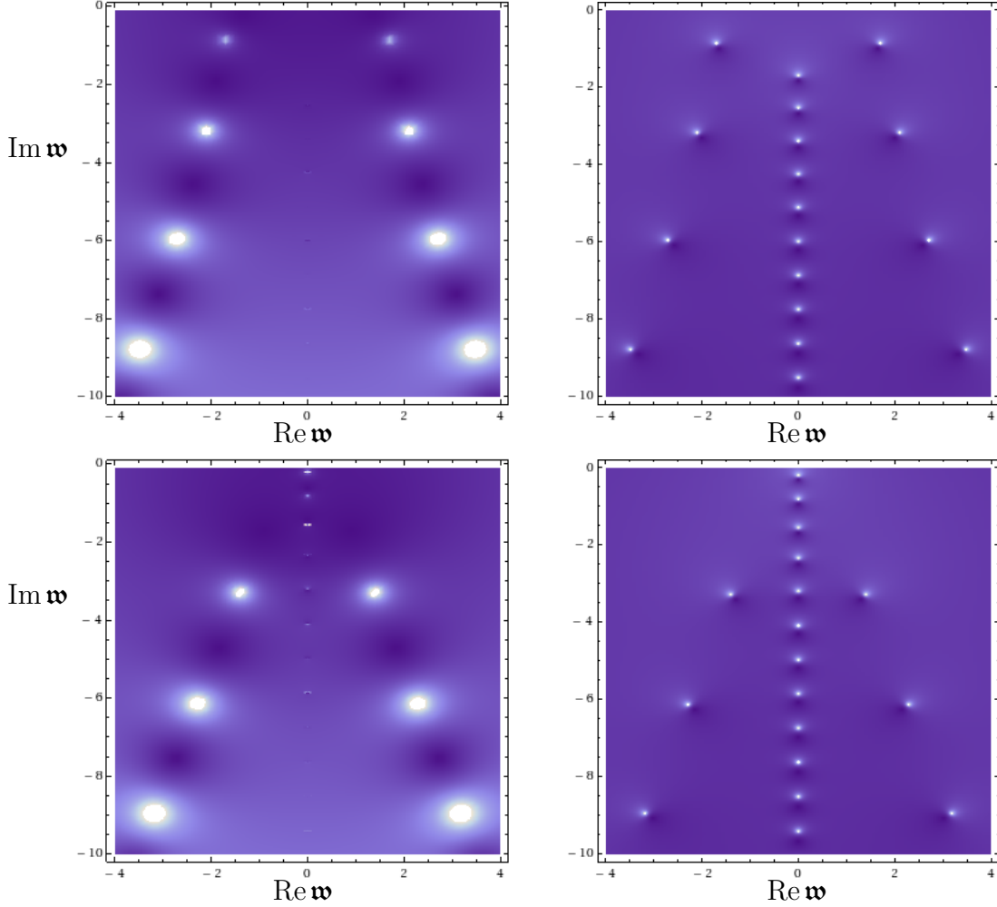
Fig. 2.1: A comparison between density plots of |\Pi_{\pm}| on the complex \mathfrak{w} plane (left panels) and the quasinormal frequencies for \Phi_{\pm} (right panels). The top row is for \Phi_{+} and the bottom row is for \Phi_{-} . All plots have \mathfrak{q} = 1 and T/\mu = 0.09 . As we discuss later, the on-axis modes are weaker but have been tested thoroughly against the quasinormal spectrum in a finer plot.
