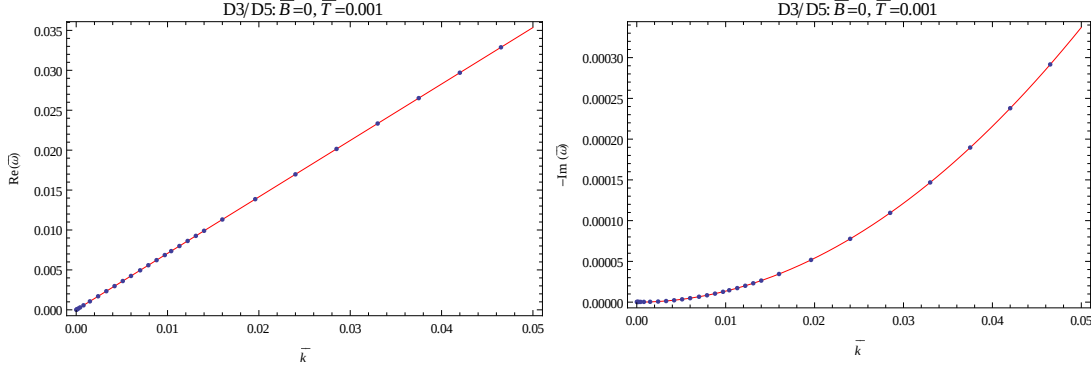
Fig. 3.2: Left: \text{Re} \bar{\omega} as a function of \bar{k} for the holographic zero sound dispersion relation in the D3/D5 system at B = 0 and \bar{T} = 0.001 , within the range \bar{T}^2 \ll \bar{T} \ll \bar{k} . Right: -\text{Im} \bar{\omega} versus \bar{k} for the same mode at the same \bar{T} . In both figures the dots are our numerical results while the red lines come from the T = 0 dispersion relation in (3.31). Clearly the T = 0 result in (3.31) is a very good approximation to our numerical results for the low-temperature dispersion relation.
