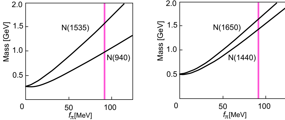
Fig. 1. The nucleon masses as functions of \langle \sigma \rangle_0 .
