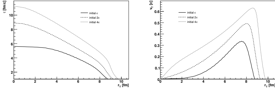
Fig. 4. Left: The typical freeze-out hypersurfaces with the fixed f.o. energy density presented in \tau - r plane for Bjorken-like azimuthally symmetric hydrodynamic expansion with equation of state P = \epsilon/3 and zero initial transverse flow. The curves correspond to the different initial energy densities \epsilon_i(\tau_i, y, r) = \epsilon_0(\tau_i, y, r) , 2\epsilon_0(\tau_i, y, r) , 4\epsilon_0(\tau_i, y, r) distributed in r -plane according to the Woods-Saxon formula. The initial proper time is \tau_i = 1 fm/c. Right: The transverse velocity distributions on freeze-out for different initial energy densities correspondingly to the left panel [37].
