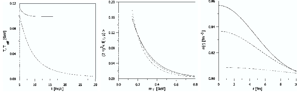
Fig. 2. Left: Evolution of the pion effective temperature T_{\text{eff}} (solid line) versus the temperature of the system T (dashed line) in the non-relativistic one-component Bjorken-like model with transverse expansion. The plots correspond to initial conditions: T_0 = 0.1 GeV, time t_0 = 5 fm/c, transverse radius R_0 = 5 fm and the initial transverse flow \hat{R}(t_0) = 0.3 . Middle and right: The pion APSD \langle f(\tau, p) \rangle (middle) and the pion densities n(r) (right) taken at typical proper times: at hadronization, \tau = 7.24 fm/c, (solid line) and at kinetic freeze-out \tau = 8.9 fm/c (dashed line). The dot-dashed line corresponds to the “asymptotic” time \tau = 15 fm/c of hydrodynamic evolution. The initial conditions of hydrodynamic expansion of hadron-resonance gas are taken from Ref. [19].
