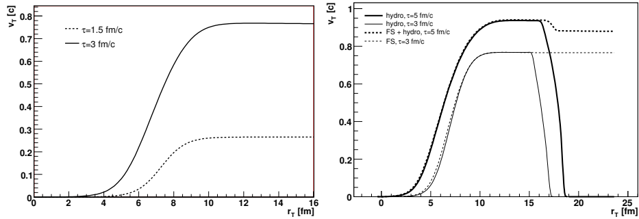
Fig. 7. Left: The collective transverse velocities (according to Ekkart \approx Landau–Lifshitz) in weakly interacting partonic system in the approximation of free streaming. The initial state at 1 \text{ fm}/c is supposed to be quasi-thermal and corresponds to the distribution (24). Dashed curve corresponds to \tau=1.5 \text{ fm}/c , solid line — 3 \text{ fm}/c . Right: The simulation of the transverse collective velocities of the quasi-free and almost massless partons within ideal hydrodynamics with the same initial conditions as for partonic system. The velocity is good approximated by such a hydro-evolution with extra-hard EoS P = 0.45\epsilon . Dashed curve corresponds to a weakly interacting partonic system at \tau=3 \text{ fm}/c and 5 \text{ fm}/c , solid line — to hydro-evolution at corresponding proper times. [7].
