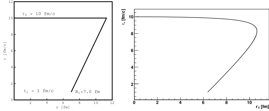
Fig. 5. Left: The parametrization of enclosed freeze-out hypersurface \tau(r) with positive r - \tau correlations. The initial proper time is \tau_i = 1 fm/c, initial collective velocity is maximal at the system border (at transverse radius r = R_i = 7 fm) and is v(R_i, \tau_i) \approx 0.34 . Right: The dynamical realization of the freeze-out with positive r - \tau correlations at constant energy density [37] based on (3 + 1)D the exact analytical solutions of relativistic hydrodynamics [38].
