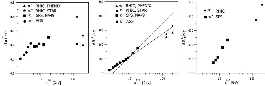
Fig. 3. Left: The average phase-space density of all negative pions at mid-rapidity, (2\pi)^3 \langle f(y) \rangle , as function of c.m. energy per nucleon in heavy ion central collisions. Middle and right: The rapidity densities of negative pions, dN^{\pi^-}/dy , and their entropy, dS^{\pi^-}/dy , as function of c.m. energy per nucleon in heavy ion central collisions [4].
