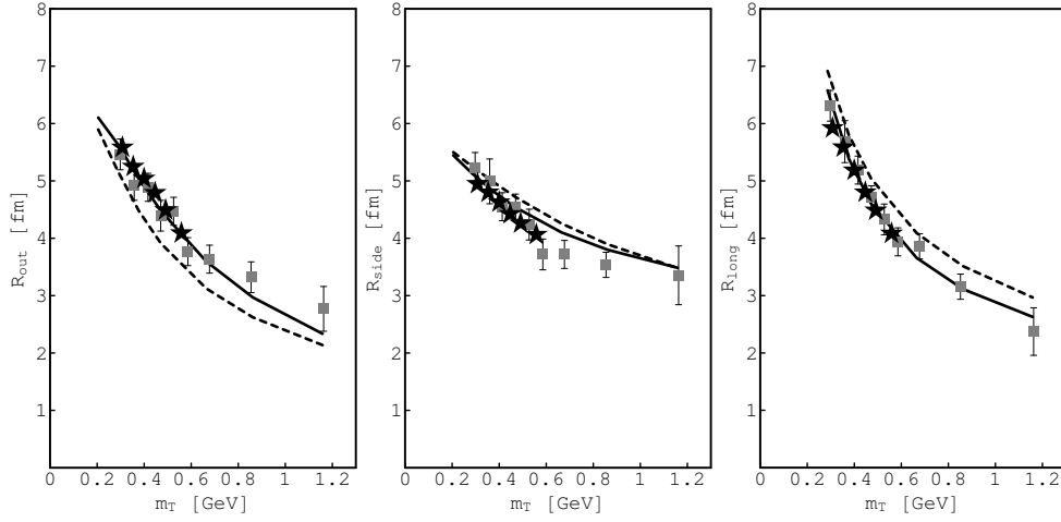
Fig. 6. Comparison of the pion source R_{out} , R_{side} , R_{long} radii measured by the STAR (stars) and PHENIX (boxes) Collaborations with model calculations performed for whole enclosed hypersurface (solid lines) and for shelf-like part only (dashed lines). The PHENIX data are adjusted for most central bin (see the text for details).
