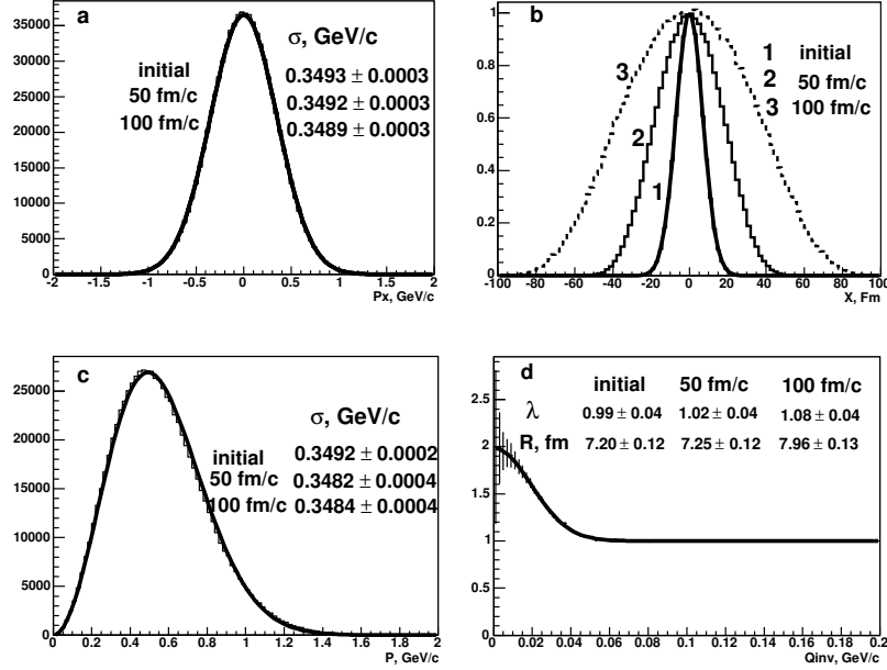
Fig.1. Distributions of the x -components of particle three-momentum (a) and three-coordinate (b), particle momentum (c) and the corresponding CF's as functions of q_{inv} (d) obtained in the UKM-R simulation of the kinetic evolution of N = 400 heavy spin-0 bosons of mass m = 0.938 GeV/ c^2 at the evolution time t = 0, 50 and 100 fm/ c . The elastic cross section \sigma_{el} = 400 mb, the initial Gaussian radius R_0 = 7 fm and the initial temperature T_0 = 0.130 GeV. Shown results of Gaussian fits of the momentum distributions and the CF's agree with the input initial values \sigma = (mT_0)^{1/2} = 0.3492 GeV/ c and \lambda = 1 , R_0 = 7 fm, respectively.
