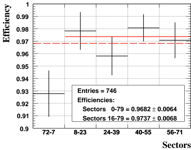
Fig. 6. Single track trigger efficiencies for tracks with p_T > 10 GeV determined for muons from Z^0 \rightarrow \mu^+\mu^- decays. Left (right) for doublet (singlet) equations.
