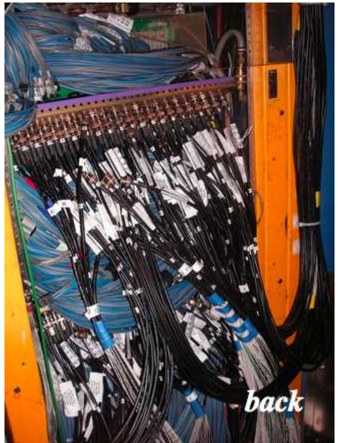
Fig. 3. The new track finding hardware installed under the DØ detector. The 40 new DFEA2 boards are arranged in 2 crates, easily accessible from the front. The 320 input and 320 output cables are located in the back of the crates.
