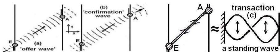
Figure 6. Cramer's Transactional Interpretation. a) Offer-wave. b) confirmation-wave combined into the resultant transaction. c) taking the form of an HD future-past advanced-retarded standing or stationary wave. Figs Adapted from Cramer [95].
