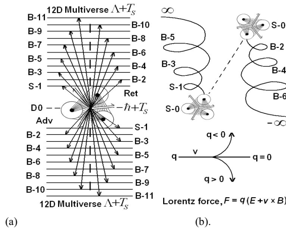
Figure 4. Conceptualized string (S) and brane (B) couplings in Advanced-Retarded spacetime arising from a least-cosmological unit D0 S-0 a) String-brane duality couplings from 0 to 12D for odd-even Fermi-Bose topologies b) Ising model spin-glass rotations which driven by an internal Lorentz-like force or external resonances for vacuum engineering.
