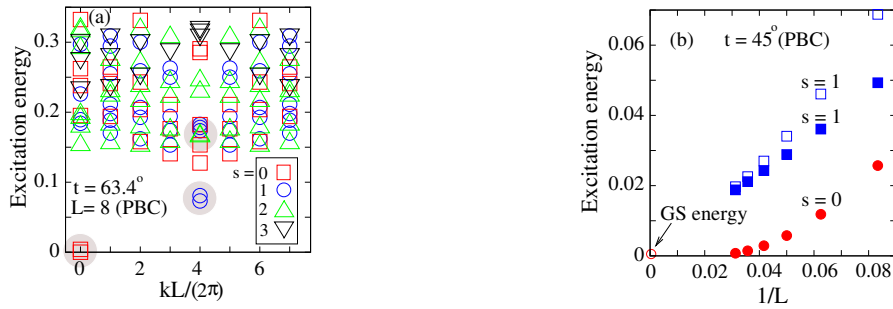
Figure 2. (a) Numerical ED results for the low-lying (spin s = 0, 1, 2, and 3 ) excitation energies of the periodic L = 8 chain at t = 63.4^\circ . The shaded symbols correspond to the lowest quasi-degenerate pairs of singlet, triplet and quintet excitations. (b) DMRG results for the FSS of the lowest singlet and triplet modes at t = 45^\circ .
