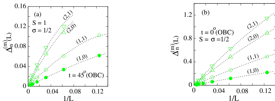
Figure 4. (a) FSS of the lowest triplet [(m, n) = (1, 0) and (1, 1)] and quintet [(m, n) = (2, 0) and (2, 1)] gaps in (a) the alternating spin (1, \frac{1}{2}) chain (DMRG, OBC, t = 45^\circ ) and (b) in the uniform (\frac{1}{2}, \frac{1}{2}) chain with 2L sites (DMRG, OBC, t = 0^\circ ). The dashed lines show the best fits to the DMRG data (symbols) obtained by Eq. (4).
