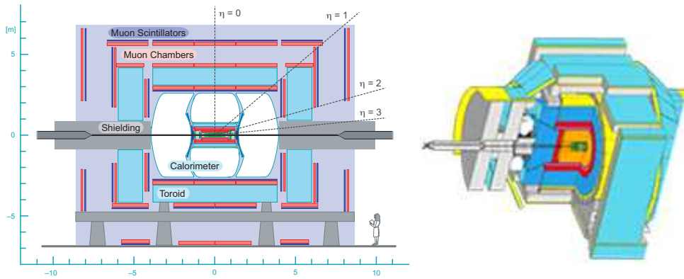
Fig. 1. The schematic view of the DØ (left) and CDF (right) detectors.
