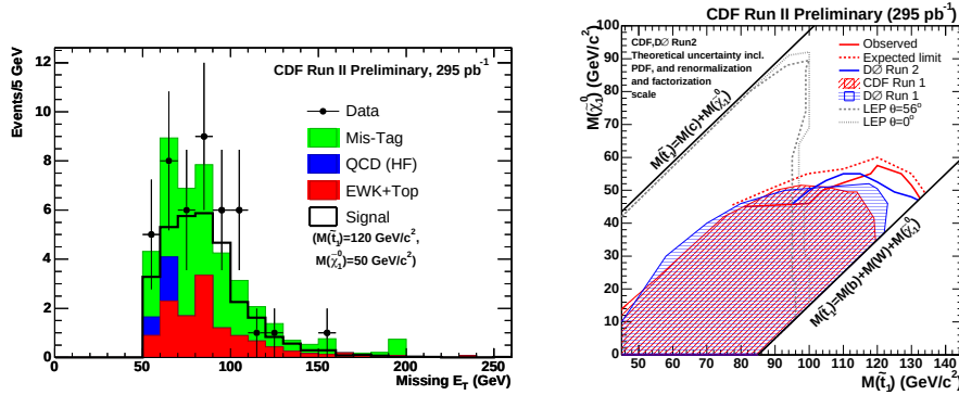
Fig. 13. MET distribution of events with at least one c -tagged jets observed by CDF together with the SM background and expected signal (left). Mass values of the lightest stop and neutralino excluded by D\bar{O} and CDF (right).
