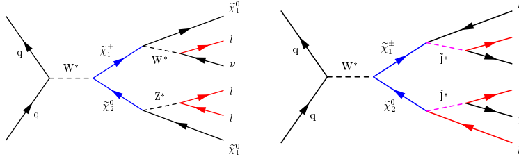
Fig. 2. Dominant production of charginos and neutralinos at the Tevatron and their decays.
