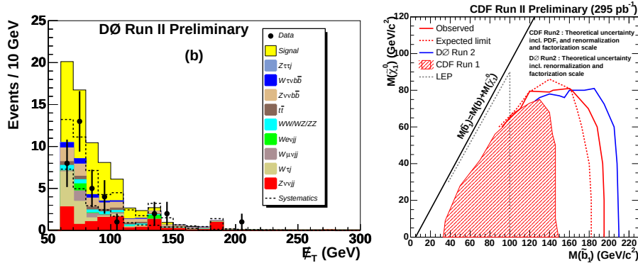
Fig. 12. MET distribution of events with at least one b -tagged jets observed by DØ together with the SM background and expected signal (left). Mass values of the sbottom and neutralino excluded by DØ and CDF (right).
