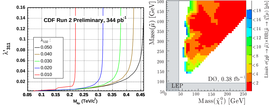
Fig. 9. Excluded regions on the plane \lambda'_{311} vs the \tilde{\nu}_\tau mass obtained by CDF (left). Cross section upper limits for the slepton mass versus the neutralino mass obtained by DØ (right).
