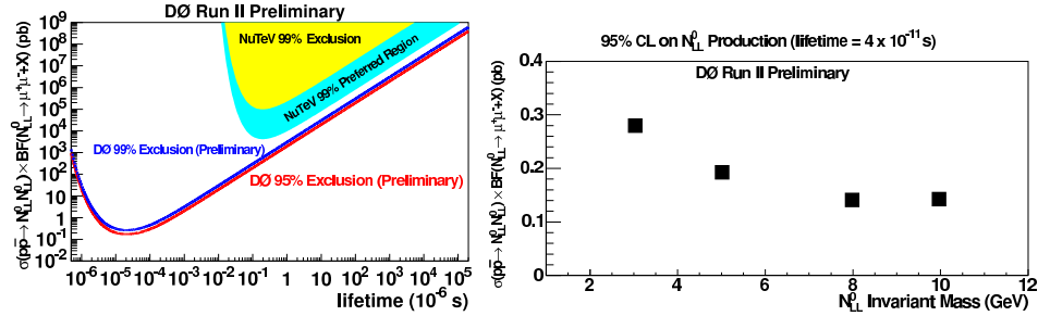
Fig. 4. 95%(99%) C.L. cross-section upper limits times branching fraction for neutral long lived (NLL) particles of mass 5 GeV as a function of its lifetime (left). The same quantity for 95% C.L. at fixed lifetime as a function of the mass of the NLL particle (right).
