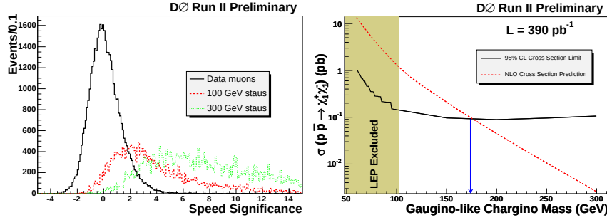
Fig. 7. Speed significance distributions of muons and of staus of two different masses. They are similar for charginos of the same mass (left). Cross section upper limit and theoretical cross-section for a gaugino-like chargino as a function of its mass (right).
