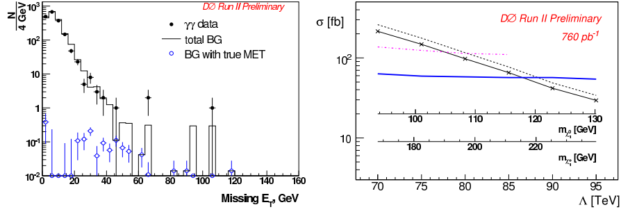
Fig. 5. MET distribution of recent DØ data (full circles), that of the background (histogram) and a part of the latter with true MET (open circles) of events containing 2 photons (left). Cross section upper limits (solid blue line) and theoretical LO (NLO) cross-section for the GMSB process (solid (dotted) black lines) (right).
