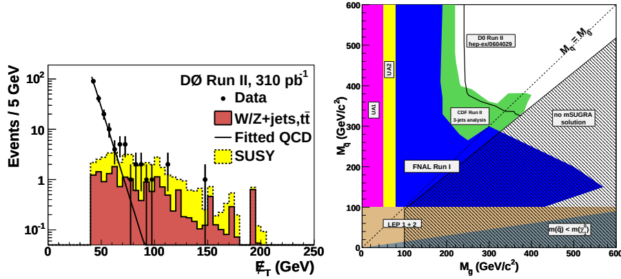
Fig. 10. MET distribution obtained by DØ for the 4-jet event topology and compared with the SM background and the expected SUSY signal (left). Excluded regions in the (M_{\text{gl}}, M_{\text{sq}}) plane obtained by CDF and DØ (right). It should be noted that DØ has used conservatively a theoretical cross-section reduced by its uncertainty.
