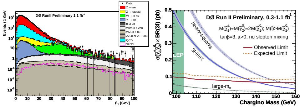
Fig. 3. MET distribution at the preselection stage of e\bar{e}l events selected by DØ (left). Cross section upper limits times branching fraction of chargino and neutralino production measured by DØ along with theoretical predictions (right).
