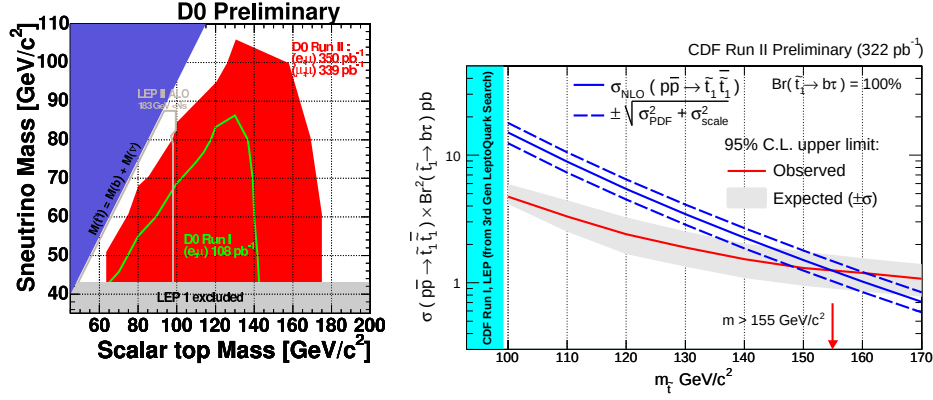
Fig. 14. Excluded regions of the stop and sneutrino masses obtained by DØ assuming the decay \tilde{t}_1 \rightarrow l + b + \tilde{\nu} , ( l = e, \mu ) (left). Upper limits of cross-section times branching fraction as a function of the stop mass obtained by CDF assuming the decay \tilde{t}_1 \rightarrow b + \tau (right). Also shown is the theoretical function.
