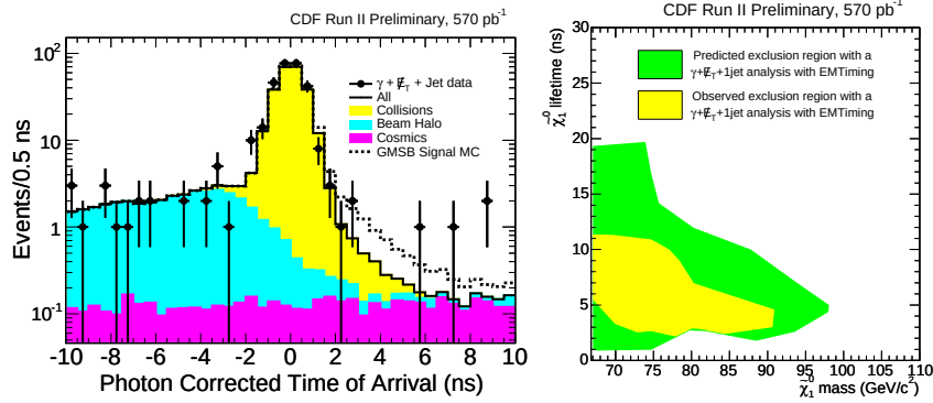
Fig. 6. Photon arrival time distribution in the CDF calorimeter (left). Excluded mass and lifetime values of the lightest neutralino (NLSP) (right).
