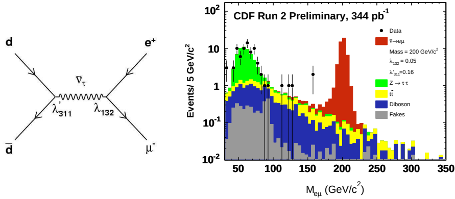
Fig. 8. RPV production and decay of \tilde{\nu}_\tau (left). Invariant mass distribution of the electron-muon pair obtained by CDF (right).
