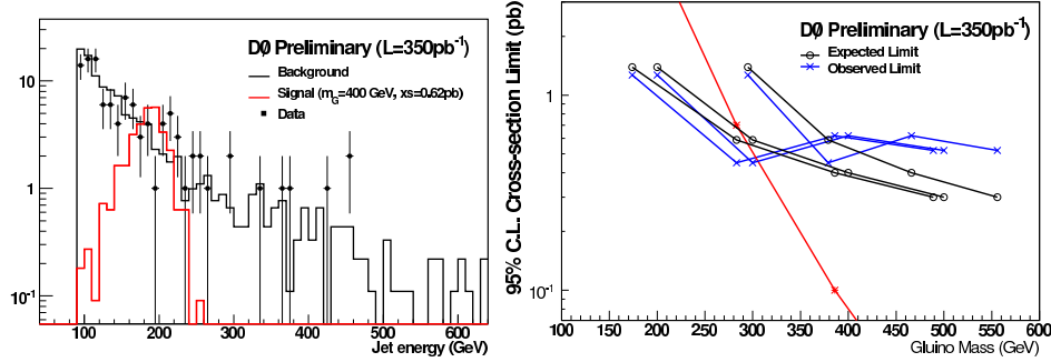
Fig. 11. Energy distribution of the selected jets (dots with error bars), that of the background (black histogram) and of a gluino of mass 400 GeV decaying into a gluon and a neutralino of mass of 90 GeV (left). Expected and observed cross-section upper limits as a function of the gluino mass for neutralino masses of 50, 90 and 200 GeV (right). Also shown is the theoretical cross-section (red star).
