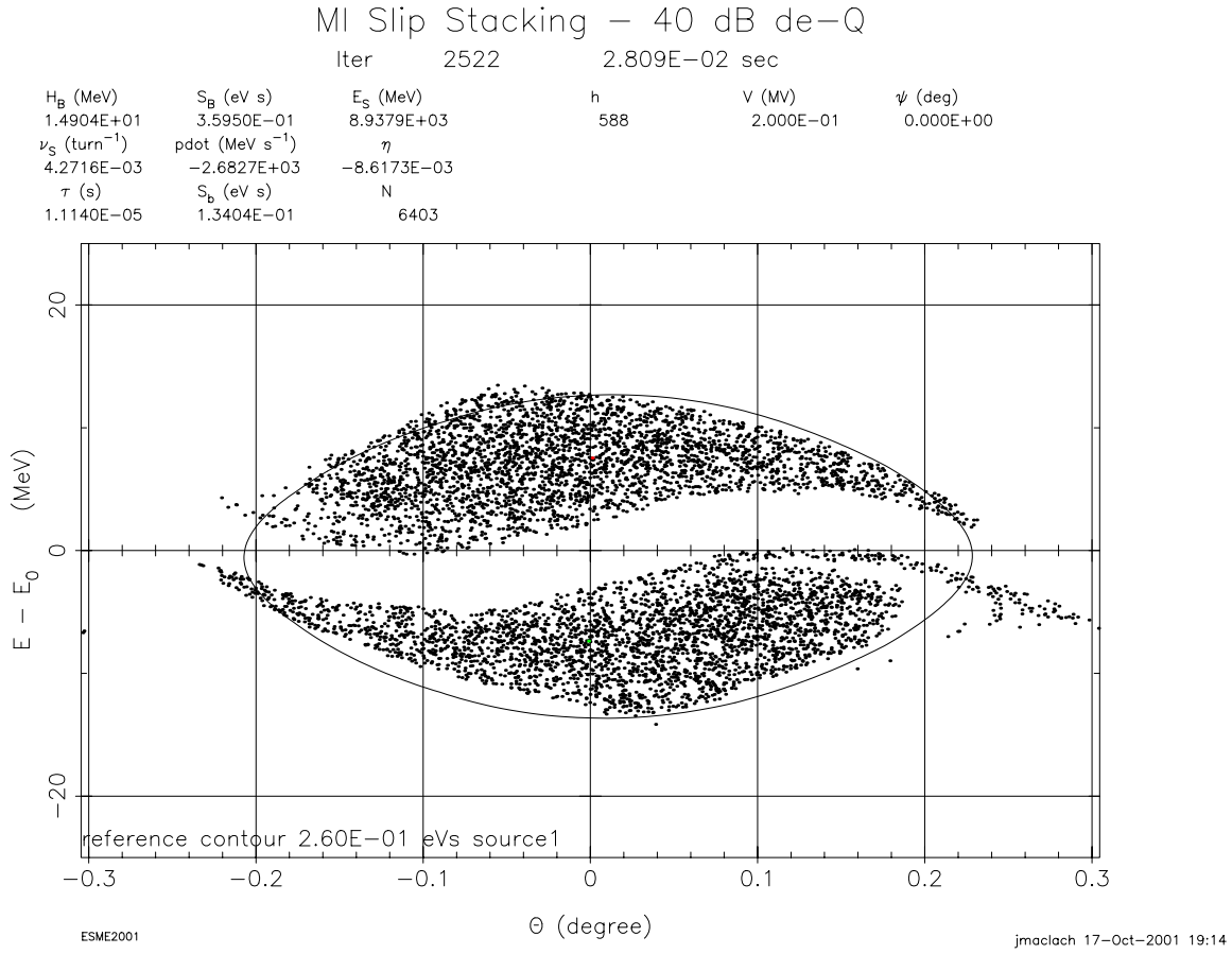
Figure 5: Comparable to Figs. 1,3, and 4, except that the MI cavities are de-Q'ed corresponding to ideal feedback with gain of 101. A matched contour of 0.26 eVs contains 95 % of the bunch.
