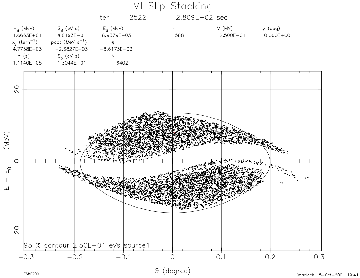
Figure 3: Comparable to Fig. 1 except that the beam loading voltage is reduced to 1/25 of the value it has naturally, corresponding to a highly idealized correction of 28 dB. A matched contour of 0.25 eVs contains 95 % of the bunch.
