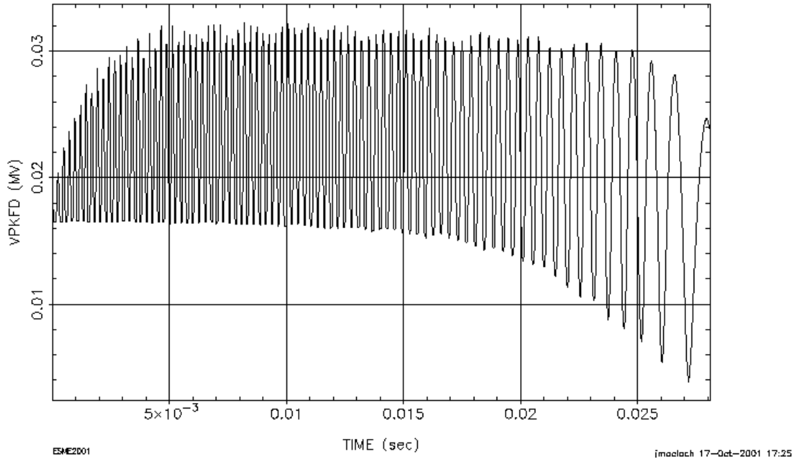
Figure 6: The beam loading voltage [MV] vs. time [s] during slip stacking with 40 dB feedback compensation; from the calculation which gave Fig. 5 for the combined bunch.
