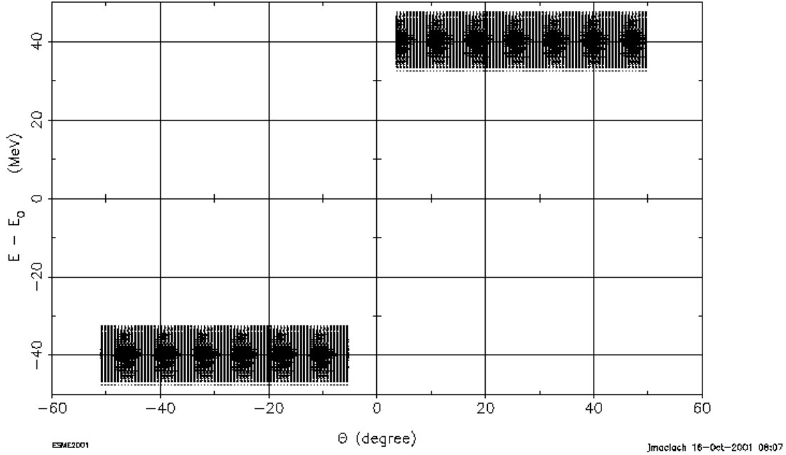
Figure 2: The initial distribution consisting of two 83 bunch batches separated in energy by 80 MeV. It is used in all of the following illustrations of the effect of the beam loading on slip stacking results.
