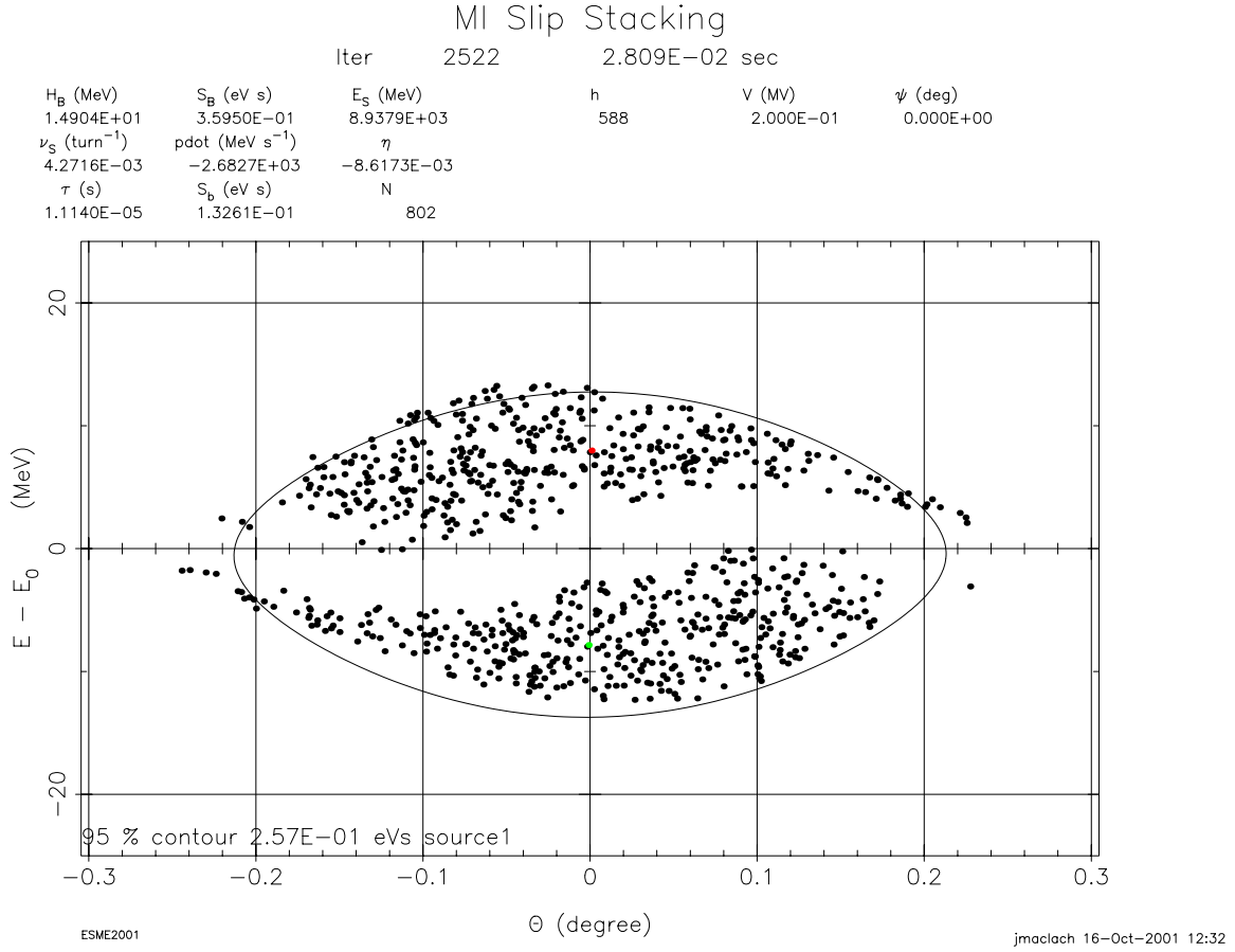
Figure 1: Single particle dynamics result for the phase space distribution for two bunches of 0.1 eVs combined by slip stacking. Machine and beam parameters are detailed in Table 2. Axes are rf phase divided by harmonic number (abscissa) and energy [MeV] with the origin on the central orbit (ordinate). 95 % of the bunch is within a matched contour of 0.26 eVs.
