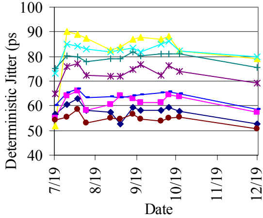
Fig. 3.1 Deterministic Jitter
