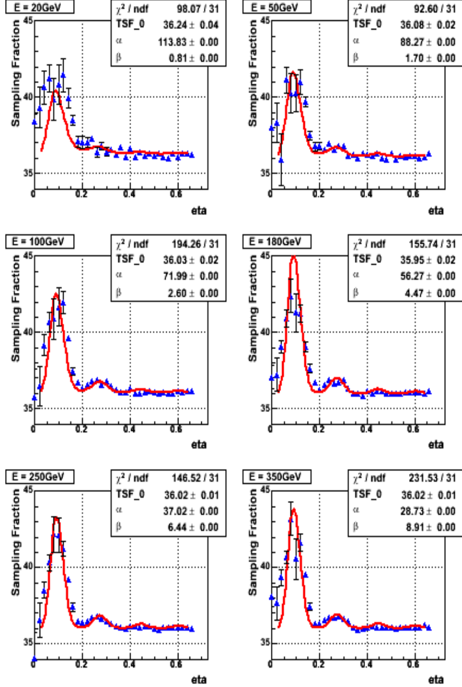
Figure 8: \text{TSF}_{\text{mean}} dependencies on \eta for different beam energies and corresponding fits by formula 4.
