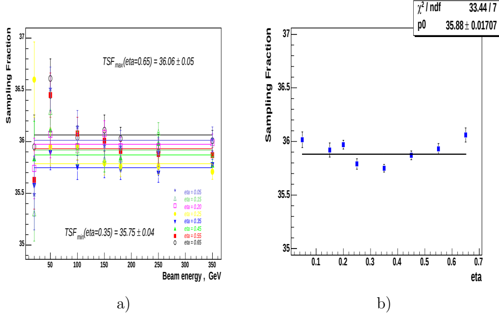
Figure 11: a) TSF dependence on beam energies for \eta -region 0.05 \div 0.65 . b) TSF averaged over beam energies for the same \eta -region.
